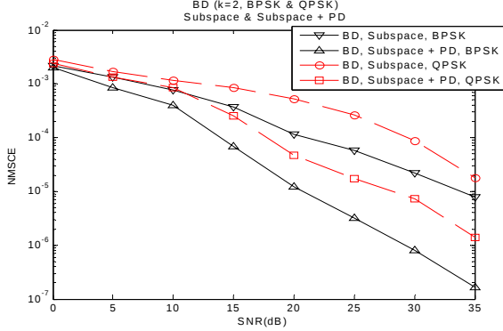
Fig. 6. Improved performances by the phase-direct technique
