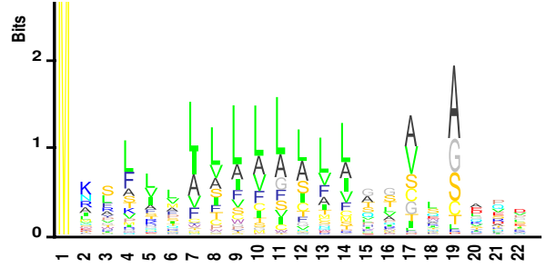
Fig. 1. Logo diagram of 179 signal peptides with cleavage site between Positions 19 and 20. Positions preceding to the cleavage site are rich in hydrophobic (e.g. A and L) and polar (e.g. G and S) residues. The taller the letter, the more often the corresponding amino acid appears in the signal peptides.
