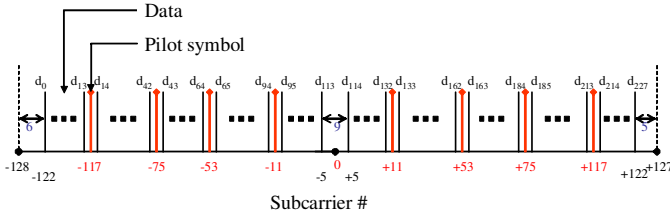
Fig. 7. Proposed data and pilot subcarriers allocation on OFDM symbol.
