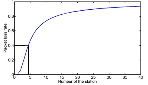
Fig. 7 Dependence of total packet loss on number of station, \lambda=37
