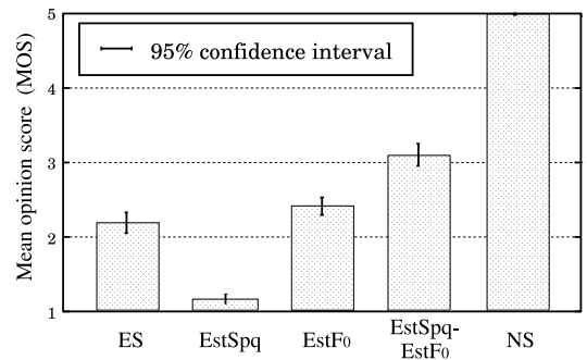
Fig. 5. Mean opinion score on naturalness.
