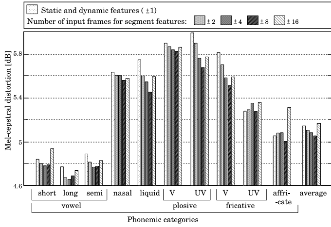
Fig. 3. Estimation accuracy of mel-cepstrum. The notation “V” denotes voiced phonemes, and “UV” denotes unvoiced phonemes.
