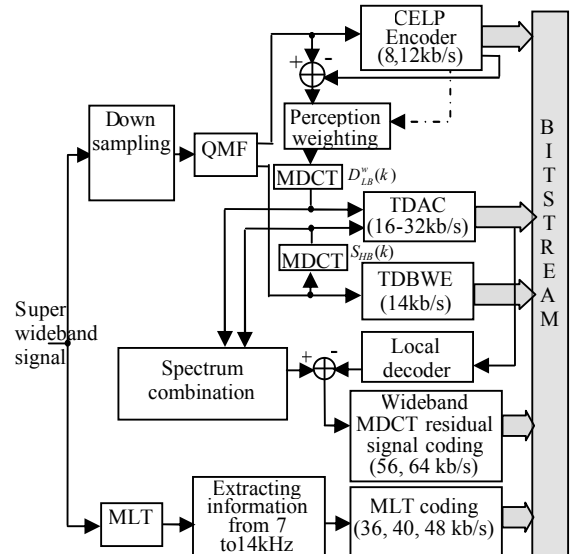
Fig. 1 Block diagram of the encoder
