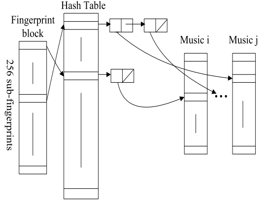
Fig. 3. Database matching stage of the PRH algorithm
