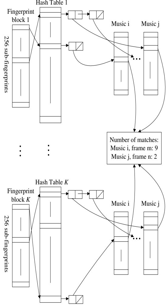
Fig. 5. Database matching stage of the SEH algorithm
