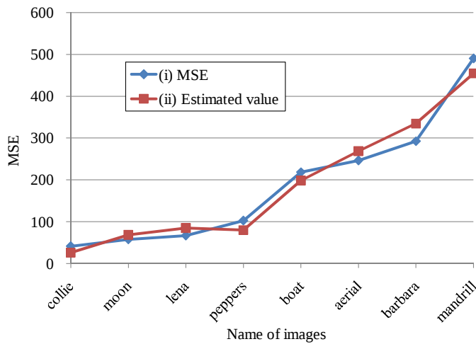
Fig. 5. MSEs of the compressed images and the estimated MSEs by the proposed method
