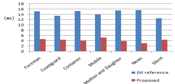
Fig. 4 Processing time comparison between the proposed method and the JM reference.
