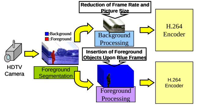
Fig. 2. Background Separation Coding.
