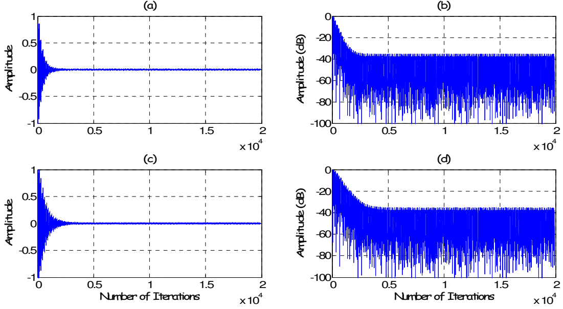
Fig. 6: Simulation results in case 1. a) residual noise obtained from the proposed algorithm b) residual noise power in db obtained from the proposed algorithm c) residual noise obtained from the FxLMS algorithm d) residual noise power in db obtained from the FxLMS algorithm
