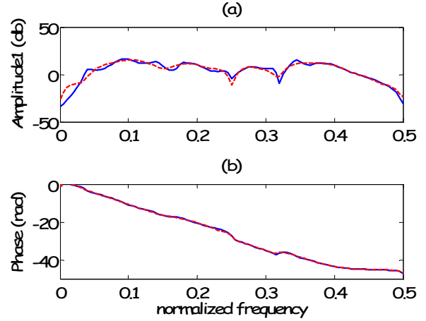
Fig. 4: Frequency response of the secondary path. a) solid: frequency response amplitude of the real system, dashed: frequency response amplitude of the estimated system. b) solid: frequency response phase of the real system, dashed: frequency response phases of the estimated system
