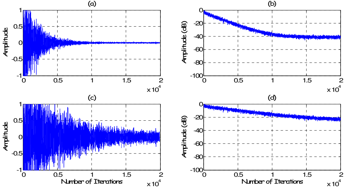
Fig. 7: Simulation results in case 2. a) residual noise obtained from the proposed algorithm b) MSE in db obtained from the proposed algorithm c) residual noise obtained from the FxLMS algorithm d) MSE in db obtained from the FxLMS algorithm
