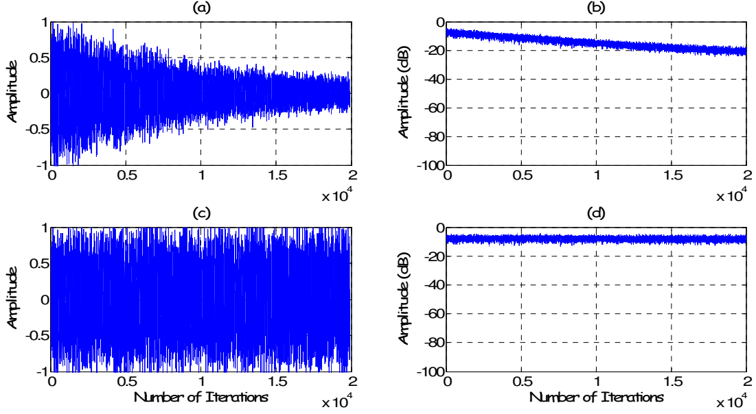
Fig. 8: Simulation results in case 3. a) residual noise obtained from the proposed algorithm b) MSE in db obtained from the proposed algorithm c) residual noise obtained from the FxLMS algorithm d) MSE in db obtained from the FxLMS algorithm
