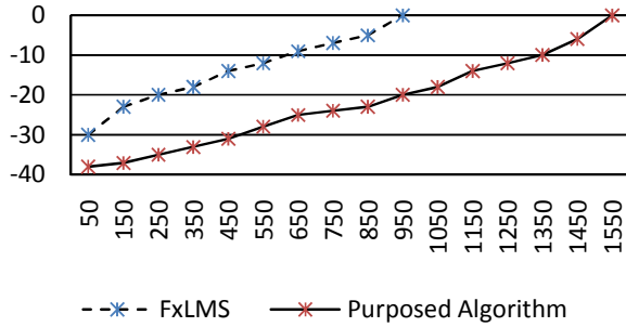
Fig. 9: Attenuation of the proposed algorithm (solid line) and the FxLMS (dashed line) with different noise band width
