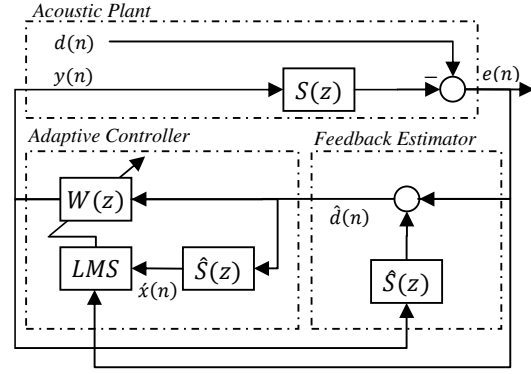
Fig. 2: Available implementation of adaptive feedback ANC
