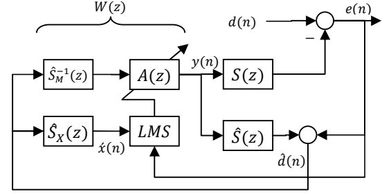
Fig. 3: The proposed structure for adaptive feedback ANC
