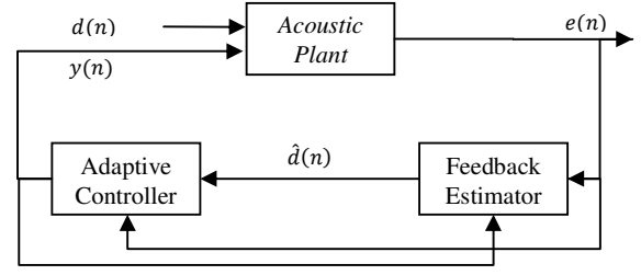
Fig.1 : General block diagram of adaptive feedback ANC
