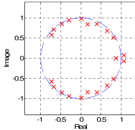
Fig. 5: Root locus of the optimal feedback ANC controller
