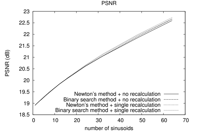
Fig. 1. PSNR of resynthesized sinusoids
