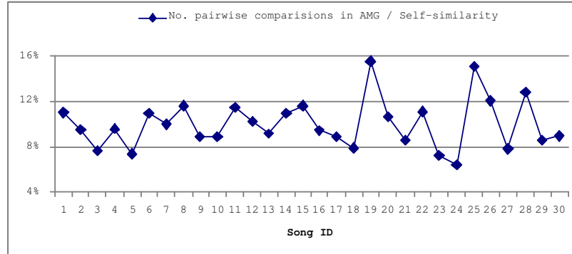
Fig. 7. The above figure compares the computational requirements between the AMG and self-similarity approach for each individual song.
