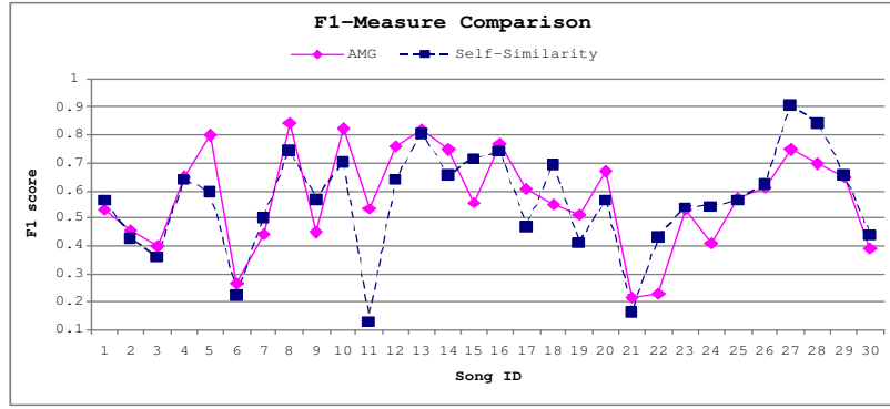
Fig. 5. The F1-measure for each individual song using the self-similarity matrix approach and our proposed AMG approach.
