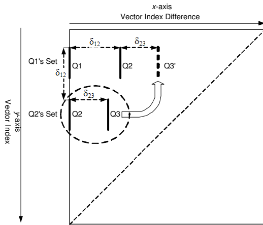
Fig. 4. The illustration of the repetition occurrence and pattern duplication process in the time-lag matrix.
