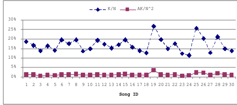
Fig. 6. The above figure compares the memory usage requirement between the AMG and self-similarity approach for each individual song. The average memory requirement of AMG is approximately 2% of that required by the self-similarity approach. The ratio K/N is also plotted to illustrate the number of branches created for each song.
