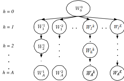
Fig. 2. The resulting candidate motif representation with Adaptive Motif Generation algorithm.
