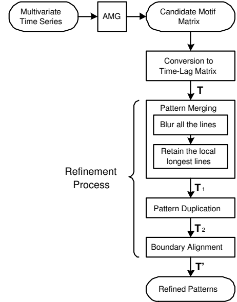
Fig. 3. The proposed process to refine the candidate motifs obtained by AMG algorithm.
