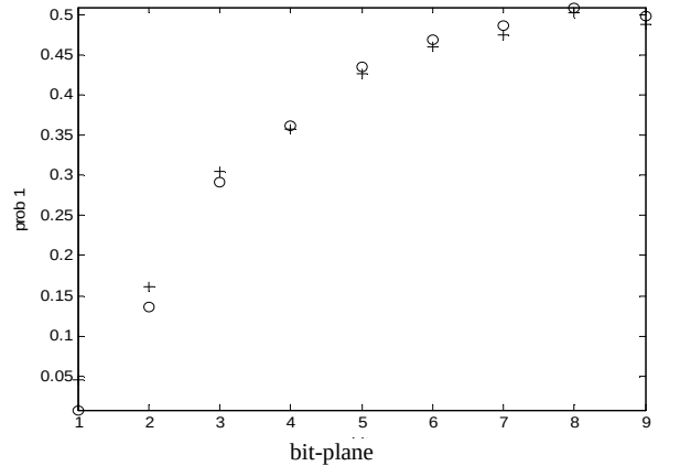
Fig. 4 Estimated probabilities of 1-bit for the HH_2 subband of Fig. 5(a), from the most significant bit-plane to the least significant bit-plane, by counting the number of 1-bits (circle symbols) and by using the proposed method (plus symbols)
