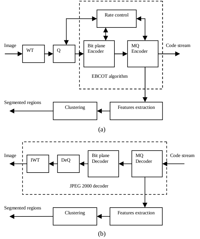
Fig. 2 Block diagram of JPEG2000 (with features extracted for image segmentation) (a) encoder (b) decoder
