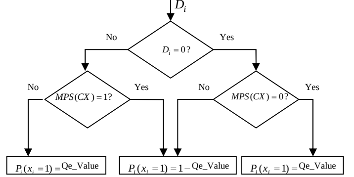
Fig. 3 Flow chart of the proposed method to estimate the local PMF: P_i(x_i = 1) on the i^{th} bit-plane; CX denotes the context of the input: D_i
