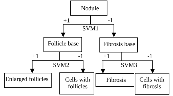
Fig. 6 Architecture of hierarchical SVM for four components.
