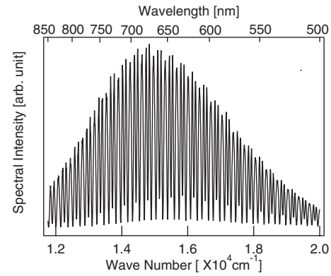
FIG. 5. Channeled spectrum P(\sigma) measured with sample C.
