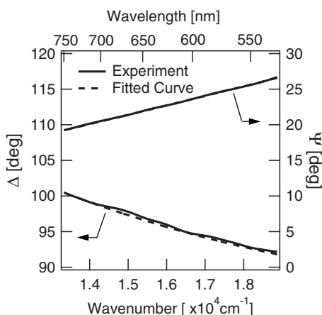
FIG. 7. Ellipsometric parameters \Psi(\sigma) and \Delta(\sigma) of sample C. Solid lines were experimentally obtained from the CSE, whereas dashed lines show the numerically fitted results by the first procedure.
