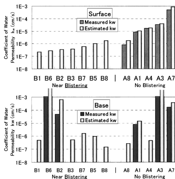
Fig. 6 Coefficient of Water Permeability k_w
