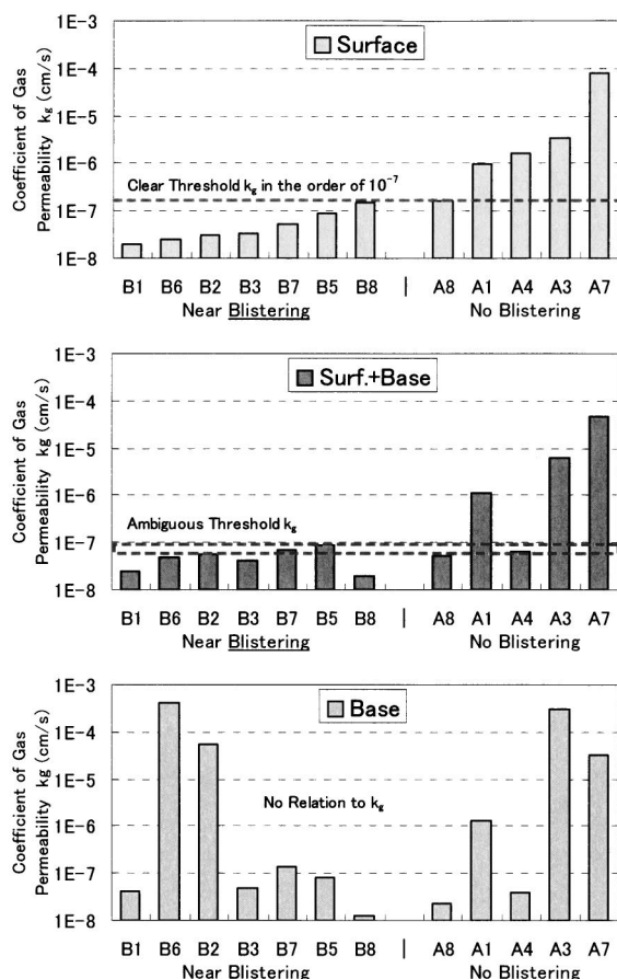
Fig. 4 Coefficient of Gas Permeability k_g
