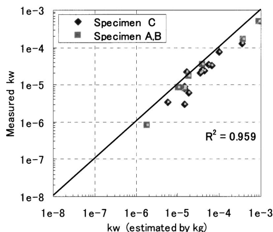
Fig. 5 Measured and Estimated Water Permeability k_w
