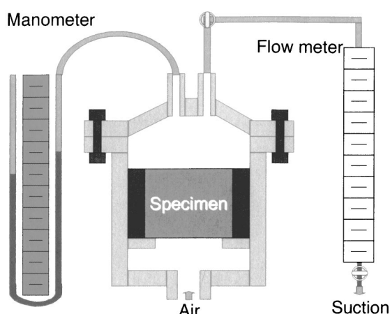
Fig. 2 Overview of Gas Permeability Tester
