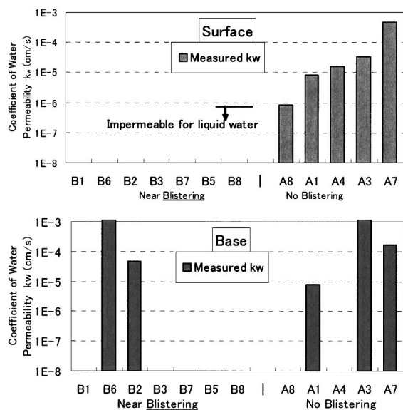
Fig. 3 Coefficient of Water Permeability k_w
