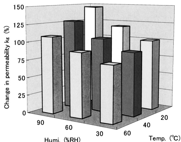
Fig. 9 Change in Permeability k_g Depending on Air Temperature and Humidity ( k_g at 20°C 30%RH = 100%)
