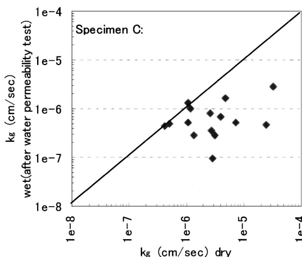
Fig. 8 Decline in Gas Permeability k_g due to Accumulated Water in Bituminous Mixtures
