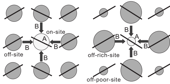
FIG. 9. Hyperfine coupling field around the molecular site. Left: non-CO state and right: fin diagonal CO state (poor on site).
