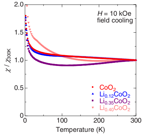
FIG. 5. (Color online) \chi-T plots for the x=0.0 (i.e., \text{CoO}_2 ), 0.12, 0.35, and 0.40 samples. In each plot, the \chi(T) values are normalized by the 300 K value.
