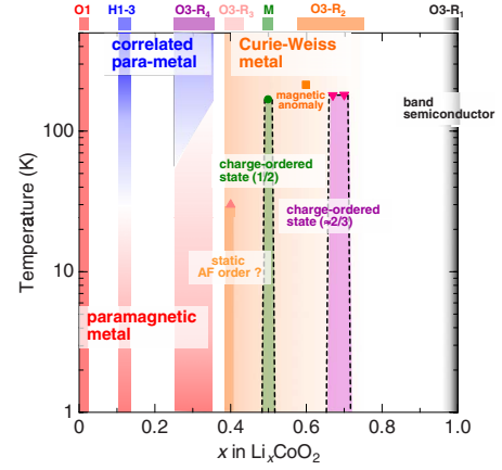
FIG. 9. (Color online) The electronic phase diagram of the \text{Li}_x\text{CoO}_2 system. The diagram has been constructed on the basis of the dc-magnetic-susceptibility data and the ^{59}\text{Co} -NMR/NQR results (Ref. 16).
