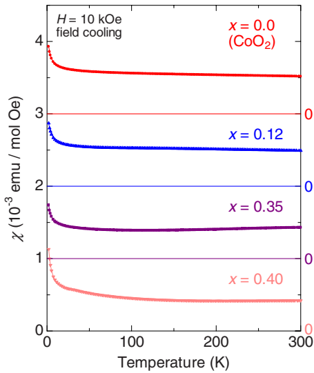
FIG. 4. (Color online) Temperature dependence of magnetic susceptibility ( \chi ) for the x=0.0 (i.e., \text{CoO}_2 ), 0.12, 0.35, and 0.40 samples. For clarity of the figure, each \chi(T) curve is shifted by 10^{-3} emu/mol Oe.
