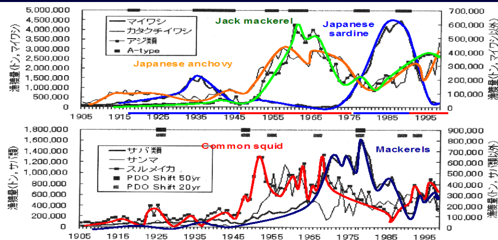
Catch fluctuations of main pelagic species for fisheries in Japan
