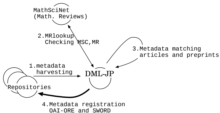
Fig. 3. Metadata registration
