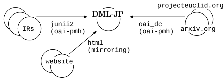
Fig. 1. Metadata harvesting
