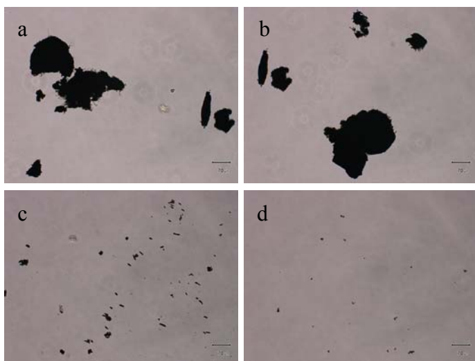
Figure 1 Light microscopic view of the loose-agglomerates (a, b) and the fine-agglomerates (c, d) of the CNTs. Aqueous suspensions containing the carbon nanotubes were mounted on glasses. Scale bars are 70 micrometers.
