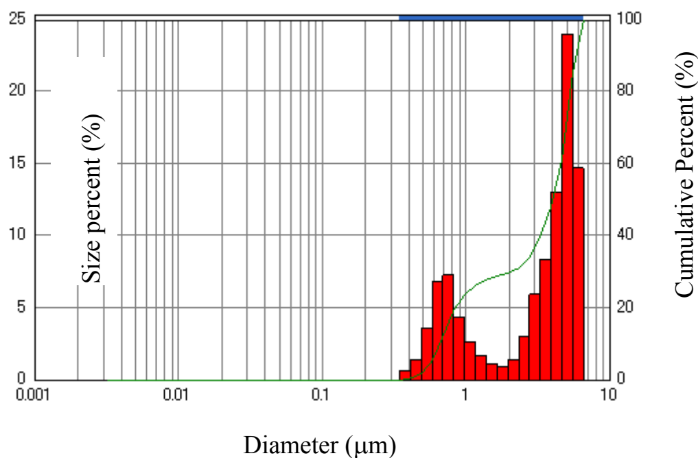
Figure 8 Dynamic light scattering size distributions of individual tubes and the agglomerates
