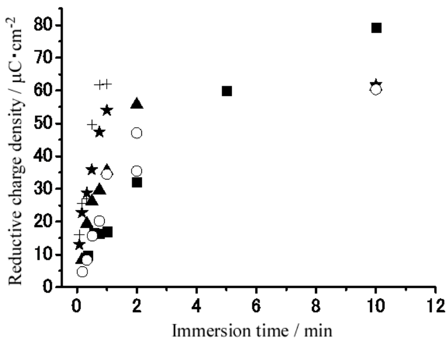
Figure 9. Reductive charge as a function of immersion time for SAMs prepared in 200 \mu\text{M} C10SH ethanol solution at 253 K (■), 261 K (○), 273 K (▲), 280 K (★), 298 K (+).
