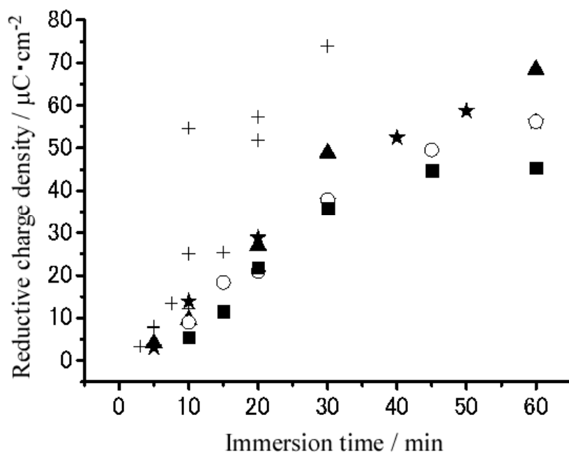
Figure 8. Reductive charge as a function of immersion time for SAMs prepared in 1 \mu\text{M} C10SH ethanol solution at 253 K (■), 261 K (○), 273 K (▲), 280 K (★), 298 K (+).
