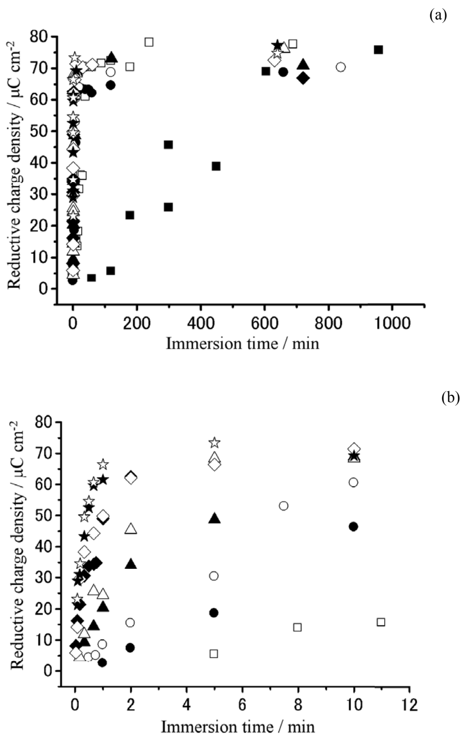
Figure 2. Reductive charge as a function of immersion time for SAMs prepared in 0.1 \mu\text{M} (■), 1 \mu\text{M} (□), 2 \mu\text{M} (●), 3 \mu\text{M} (○), 5 \mu\text{M} (▲), 10 \mu\text{M} (△), 50 \mu\text{M} (◆), 100 \mu\text{M} (◇), 200 \mu\text{M} (★), and 500 \mu\text{M} (☆) C10SH ethanol solutions at room temperature.
