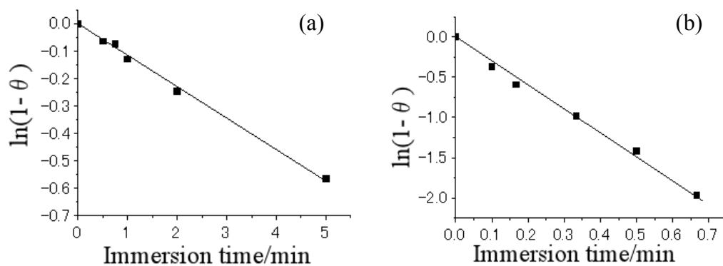
Figure 5. Immersion time dependencies of \ln(1-\theta) of SAM prepared in (a) 3 \mu\text{M} and (b) 200 \mu\text{M} C10SH ethanol solutions at room temperature.
