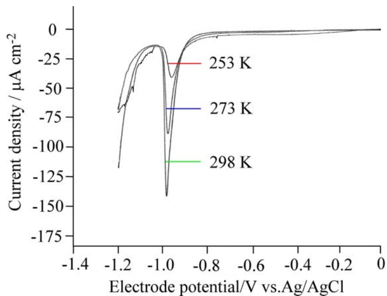
Figure 7. Current-voltage curves of Au (111) single crystal electrode, which was modified by immersing in ethanol solution containing 200 \mu\text{M} C10SH at various temperatures for 1 min, measured in 0.5 M KOH. Sweep rate : 10 mV/s.
