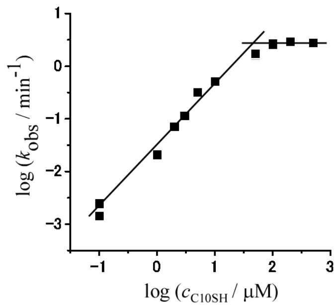
Figure 6. Relation between \log(k_{\text{obs}}) and \log(\text{concentration of C10SH}) .
