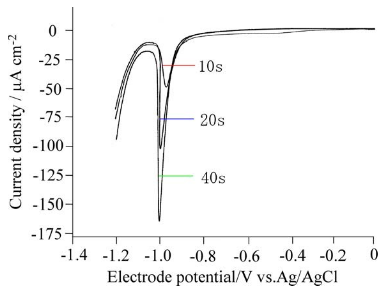
Figure 1. Current-voltage curves of Au (111) single crystal electrode, which was modified by immersing in ethanol solution containing 100 \mu\text{M} C10SH for various time periods at room temperature, measured in 0.5 M KOH. Sweep rate : 10 mV/s.
