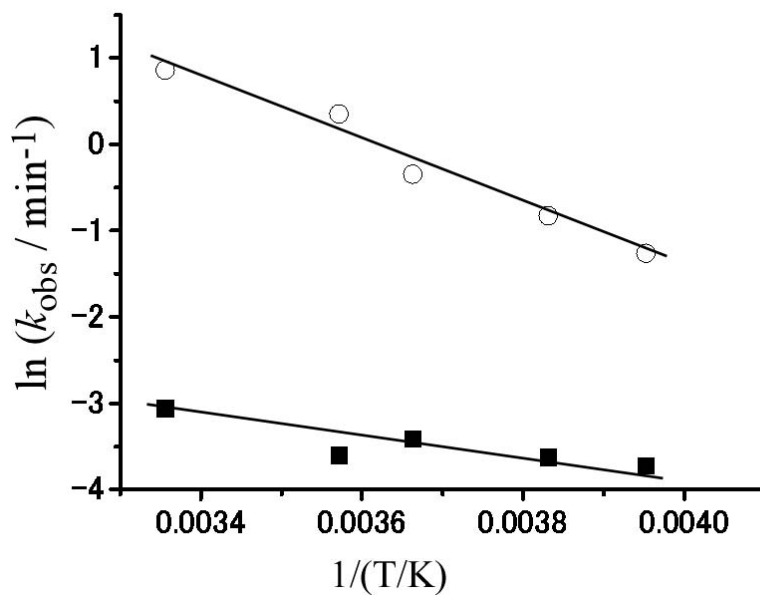
Figure 10. Temperature dependencies of the SAM formation rate constant in 1 \mu\text{M} (■) and 200 \mu\text{M} (○) C10SH ethanol solution.
