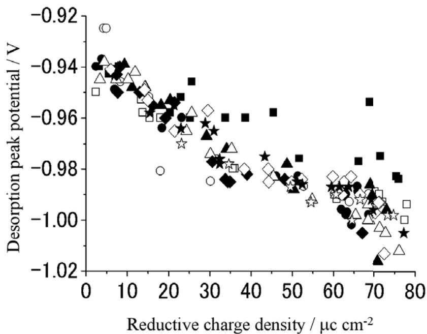
Figure 4. Relation between reductive desorption peak potentials and the reductive charge obtained for SAMs prepared in 0.1 \mu\text{M} (■), 1 \mu\text{M} (□), 2 \mu\text{M} (●), 3 \mu\text{M} (○), 5 \mu\text{M} (▲), 10 \mu\text{M} (△), 50 \mu\text{M} (◆), 100 \mu\text{M} (◇), 200 \mu\text{M} (★), and 500 \mu\text{M} (☆) C10SH ethanol solutions at room temperature.
