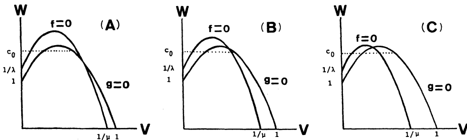
Figures 2. The curves f=0 , g=0 for different values of \lambda , \mu , \alpha .
