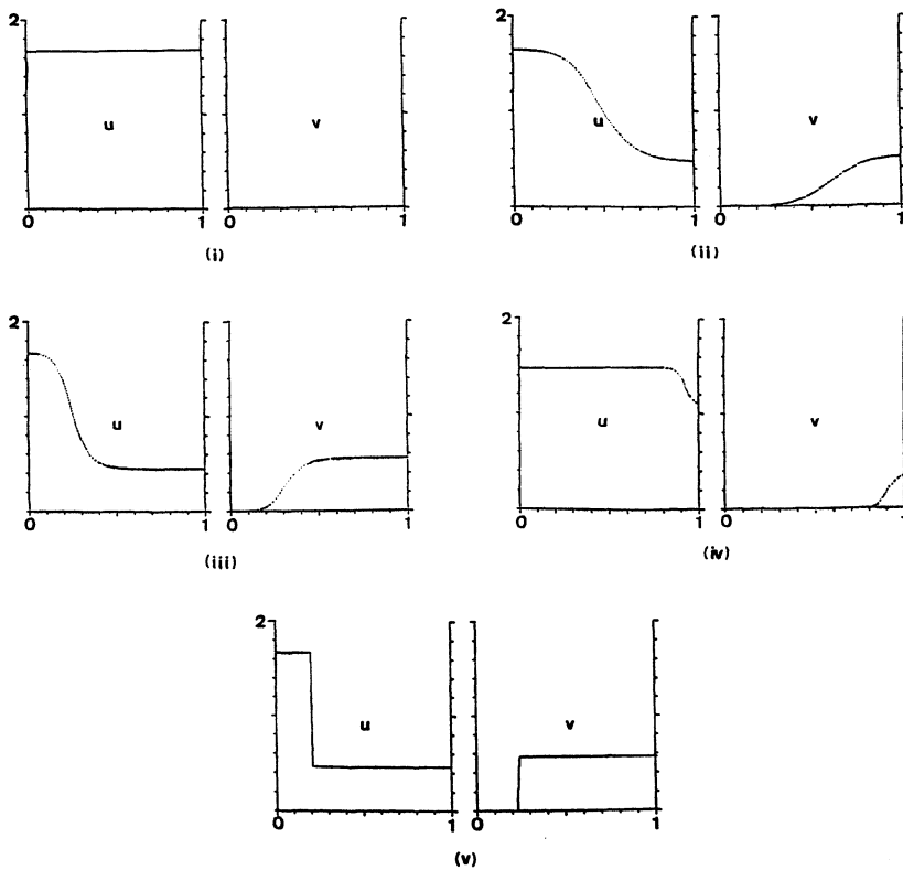
Figure 6b. Spatial patterns of u and v when D varies. \alpha=5 , \beta=1 , \lambda=0.68 , \mu=1.2 (this case corresponds to case (III)) and (i) D=0.005 , (ii) D=0.004 , (iii), (iv) D=0.001 , (v) D=0.0 .
