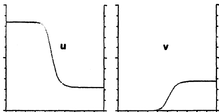
Figure 4. Internal transition layer solutions when D is small.
