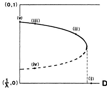
Figure 6a. The spontaneous bifurcation with respect to D . A solid line represents an internal transition layer solution and a dashed line a boundary layer one.
