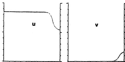
Figure 5. Boundary layer solutions when D is small.
