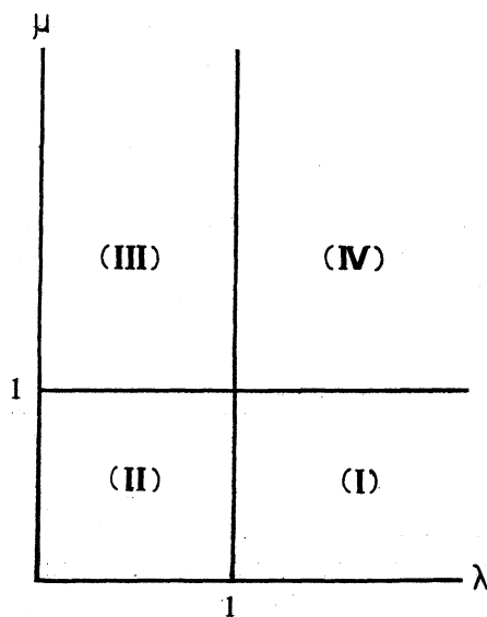
Figure 1. Classification of constant steady states of (1.1) with \alpha=0 in (\lambda, \mu) -space.
