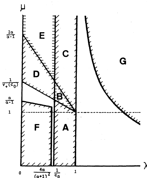
Figure 3. Existence and non-existence regions of non-constant steady states of (1.1) in (\lambda, \mu) -space.
