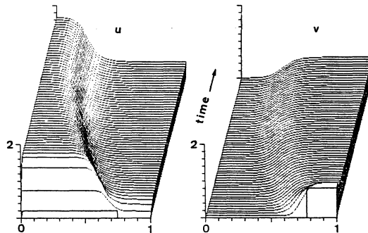
Figure 7. Spatio-temporal profiles of solution of (1.1). The values of the coefficients correspond to the case (iii) in Figure 6b.
