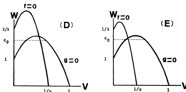
Figure 2. The curves f=0, g=0 for different values of \lambda, \mu, \alpha .
