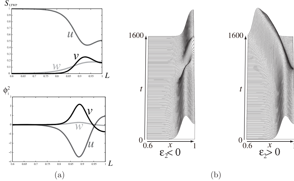
Figure 9. (a) The respective profiles of S_{LTWP} and \phi_1^2 . (b) The output patterns for a small perturbation of \phi_1^2 to S_{LTWP} . Fusion and annihilation is observed for negative and positive \epsilon_2 , respectively.
