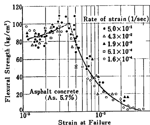
Fig. 5 Relation between Strain at Failure and Flexural Strength
