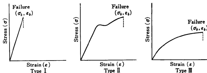
Fig. 1 Stress-Strain Relationships
