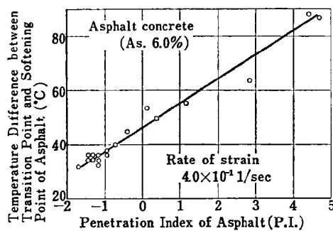
Fig. 14 Penetration Index of Asphalt vs. Temperature Difference between Transition Point of Asphalt Concrete and Softening Point of Asphalt
