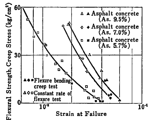
Fig. 10 Relation between Flexural Strength and Creep Stress and Strain at Failure
