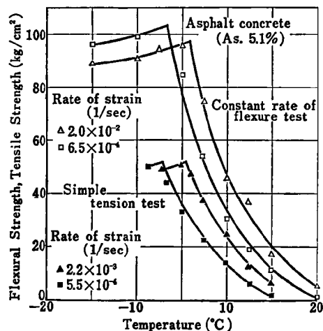
Fig. 8 Flexural Strength and Tensile Strength of Asphalt Concrete in Constant Rate of Flexure Test and Simple Tension Test
