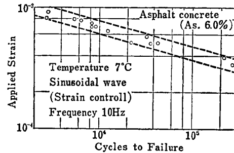
Fig. 15 Effect of Applied Strain on Cycles to Failure
