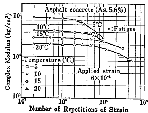
Fig. 16 Effect of Temperature on Complex Modulus and Fatigue Life
