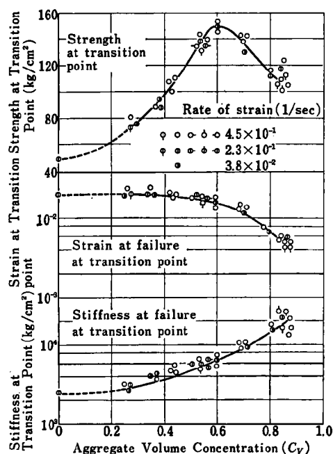
Fig. 11 Relation between Strength, Strain, and Stiffness at Transition Point and Aggregate Volume Concentration
