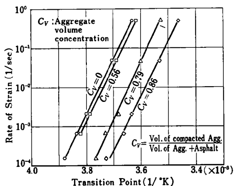
Fig. 4 Effect of Rate of Strain on Movement of Transition Point
