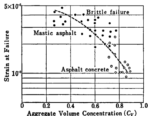
Fig. 12 Relation between Strain at Failure and Aggregate Volume Concentration
