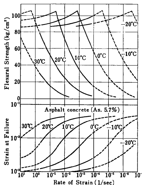
Fig. 6 Mastercurves of Flexural Strength and Strain at Failure vs. Rate of Strain
