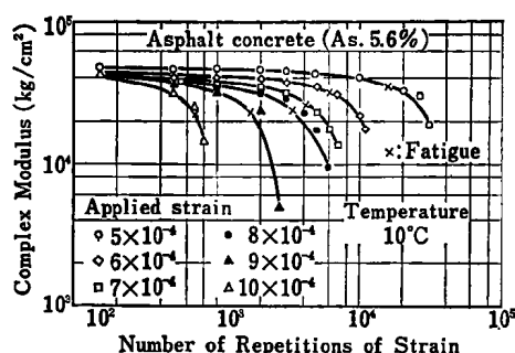
Fig. 17 Effect of Applied Strain on Complex Modulus and Fatigue Life
