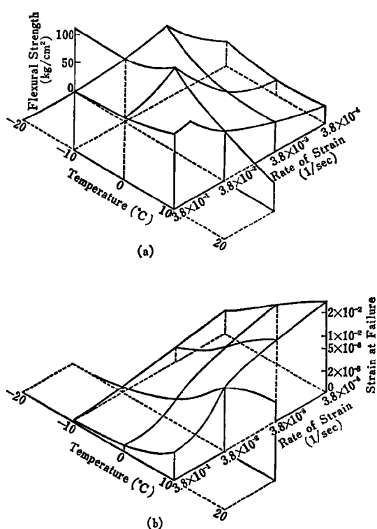
Fig. 3 Effect of Temperature and Rate of Strain on Flexural Strength and Strain at Failure (Asphalt concrete: As. 7.0%)
