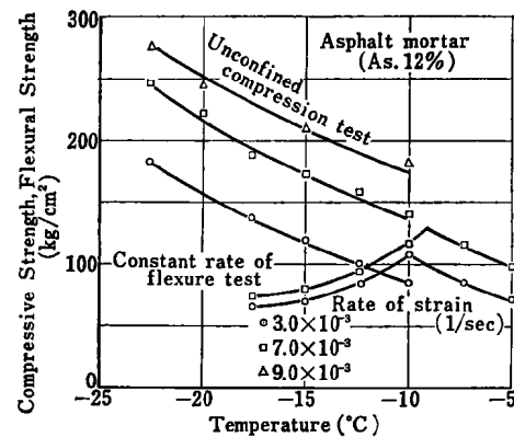
Fig. 9 Compressive Strengths and Flexural Strengths of Asphalt Mortar in Constant Rate of Flexure Test and Unconfined Compression Test
