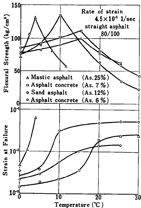
Fig. 7 Flexural Strength and Strain at Failure of Each Type of Bituminous Mixture
