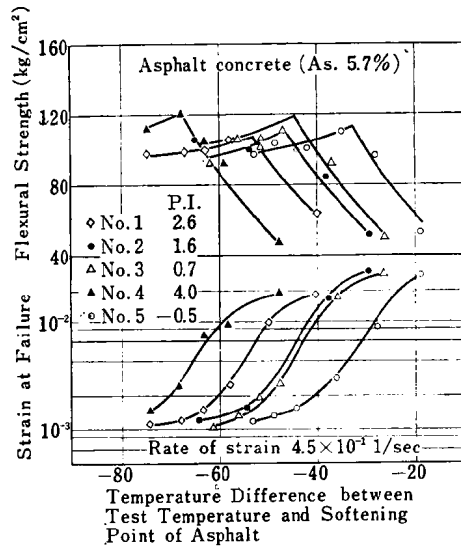
Fig. 13 Effect of Binder Property on Strain at Failure and Flexural Strength
