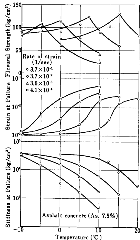
Fig. 2 Effect of Rate of Strain on Flexural Strength, Strain at Failure and Stiffness at Failure
