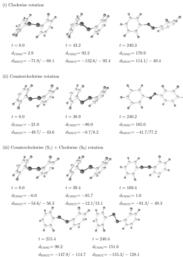
FIG. 5. Snapshots along example trajectories for (i) clockwise rotation, (ii) counterclockwise rotation, and (iii) counterclockwise ( S_1 ) + clockwise ( S_0 ) rotation, starting from cis -azobenzene.
