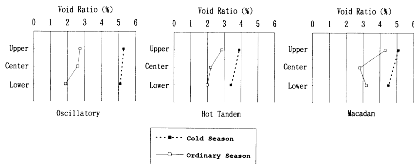
Fig. 9 Vertical Distribution of Void Ratio in First Binder Course
