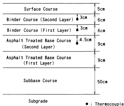
Fig. 1 Pavement Structure
