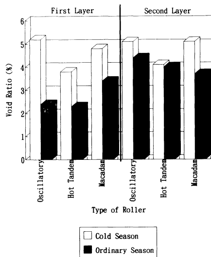
Fig. 8 Void Ratio in Binder Course
