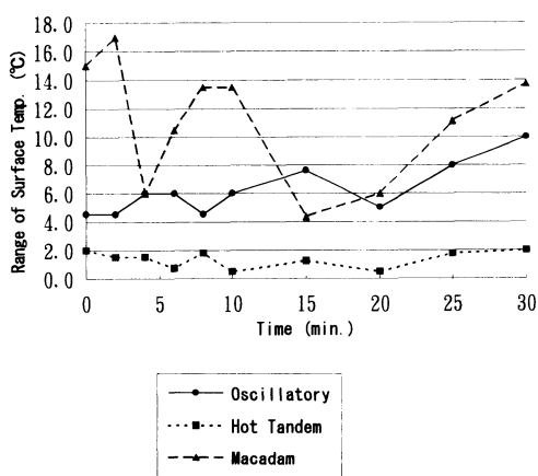
Fig. 4 Range of Surface Temperature of First Binder Course Constructed in Cold Season (Location A)
