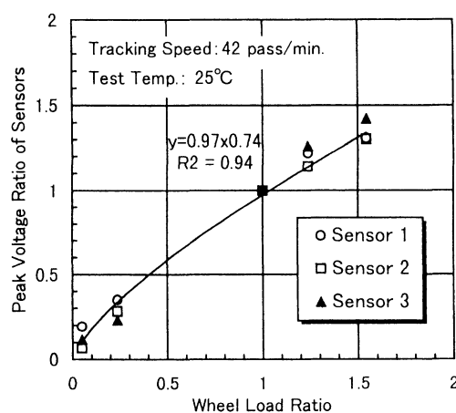
Fig. 3 Voltage of Sensor under Various Wheel Loads (at Calibration)
