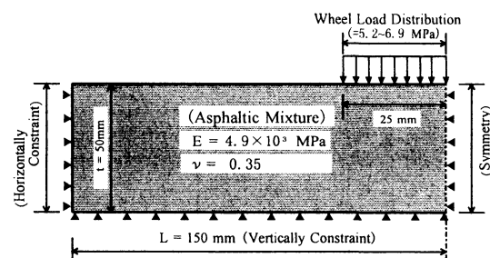
E: Elastic modulus, \nu : Poisson's ratio. FEM indicates elastic and viscoelastic analysis using finite element method.
