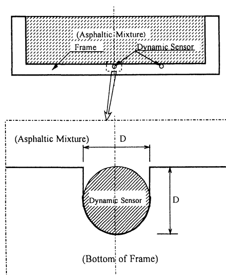
D: Diameter of dynamic sensor.
