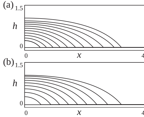
Fig. 3. Evaporation process with e = 2.5 \times 10^{-3} . In this simulation, the spatial mesh size and the temporal mesh size were taken to be 0.010 and 5.0 \times 10^{-4} , respectively. The curves in (a) and (b) represent the profile of h every 50 unit times for (a) A = 0.0 and (b) A = 0.060 .
