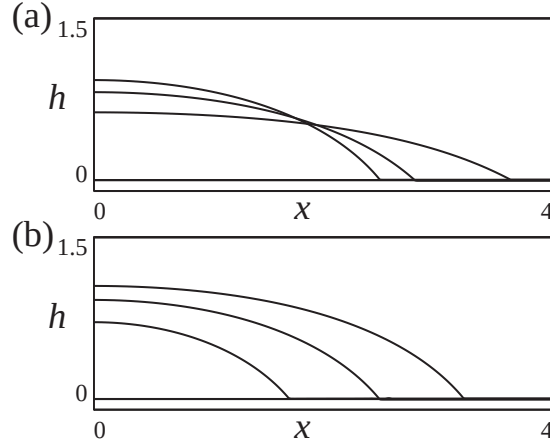
Fig. 2. The profiles of droplets z = h in the stationary states. (a) \Gamma = 0.20, 0.90, 1.6 and h_l = 1.0 . (b) \Gamma = 0.20 and h_l = 0.50, 1.0, 1.5 . In the simulations, the spatial mesh size and the temporal mesh size were taken to be 0.010 and 5.0 \times 10^{-4} , respectively.
