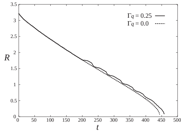
Fig. 6. Radius of droplet vs time. The dotted and solid curves correspond to Figs. 5(a) and 5(b), respectively.
