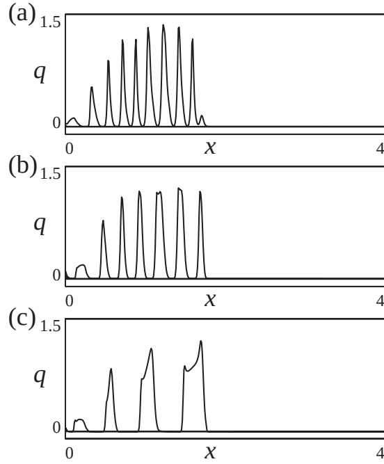
Fig. 5. The profiles of precipitation q for \Gamma_q of (a) 0.0, (b) 0.25 and (c) 1.0. In the simulations, the spatial mesh size and the temporal mesh size were taken to be 0.010 and 5.0 \times 10^{-4} , respectively. Evaporation rates are set as e = 2.5 \times 10^{-3} and A = 0.060 .
