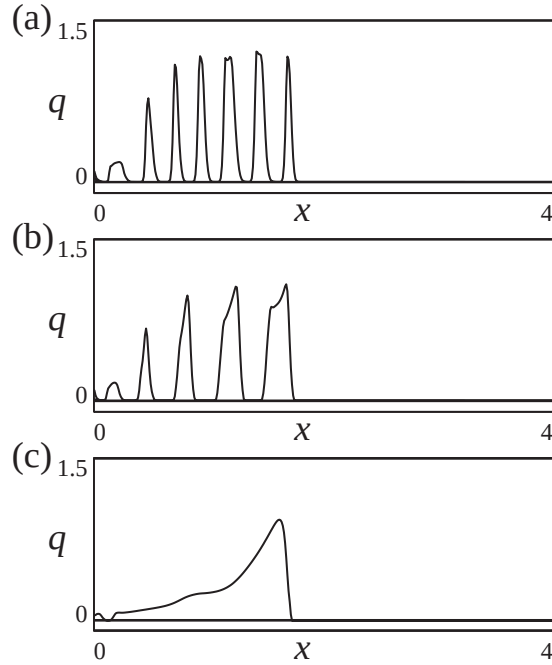
Fig. 7. The profiles of precipitation q with (a) e = 2.50 \times 10^{-3} , (b) e = 1.25 \times 10^{-3} and (c) e = 2.50 \times 10^{-4} . In the simulations, the spatial mesh size and the temporal mesh size were taken to be 0.010 and 5.0 \times 10^{-4} , respectively. Other parameters were set to be \Gamma_q = 0.25 and A = 0.060 .
