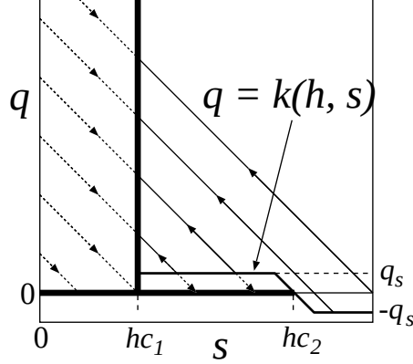
Fig. 4. Local dynamics in the s - q plane for the fixed value of h is displayed. The solid arrows indicates precipitation from supersaturated solution and the dotted one implies dissolution. The bold lines correspond to the stable ( s \leq hc_1 ) or metastable ( s > hc_1 ) states. The graph of q = k(h, s) is designed for a separatrix of the flow in the supersaturated region, where q_s is taken to be small.
