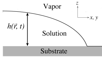
Fig. 1. The physical configuration showing the Cartesian coordinate system and describing an evaporating thin liquid film on a solid substrate.
