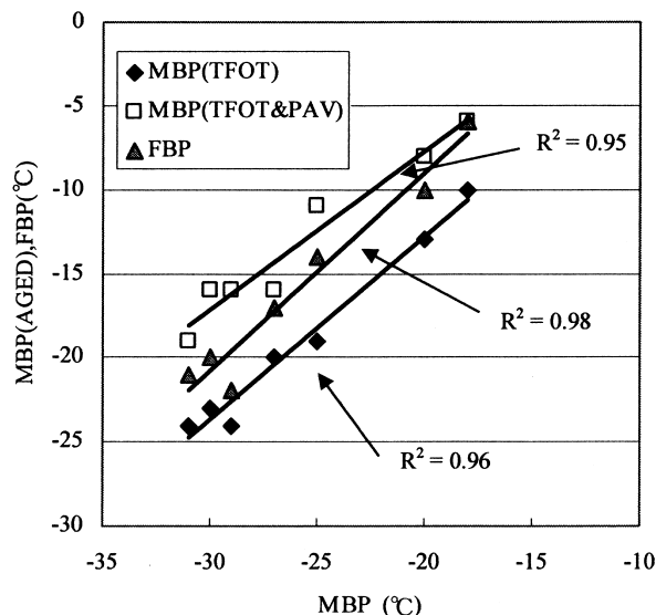
Fig. 1 Relationship between MBP (tank) and MBP (aged), FBP
