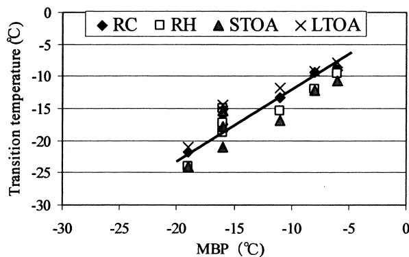
Fig. 7 Relationship between MBP and Transition Temperature of Asphalt Mixtures
