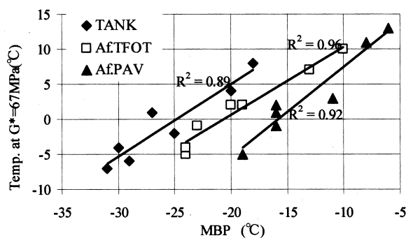
Fig. 3 Relationship between MBP and Temperatures at Limiting Stiffness from DSR
