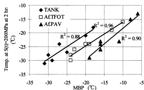
Fig. 2 Relationship between MBP and Temperatures at Limiting Stiffness from Nomograph
