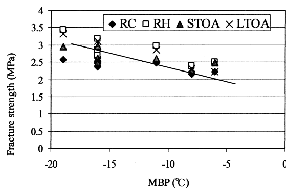
Fig. 6 Relationship between MBP and Fracture Strength of Asphalt Mixtures
