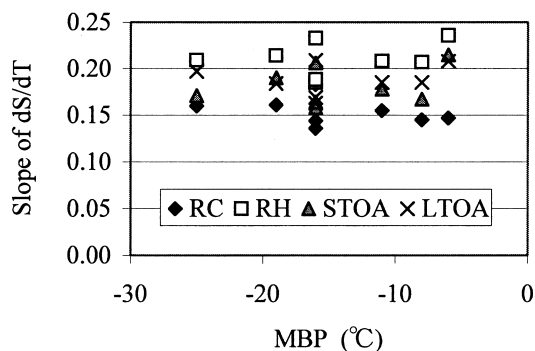
Fig. 8 Relationship between MBP and Slope of dS/dT of Asphalt Mixtures
