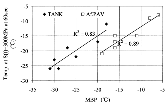
Fig. 4 Relationship between MBP and Temperatures at Limiting Stiffness from BBR
