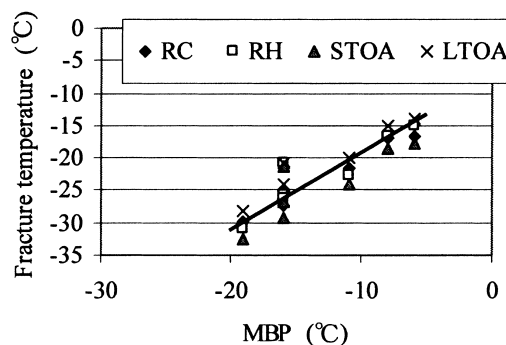
Fig. 5 Relationship between MBP and Fracture Temperatures of Asphalt Mixtures
