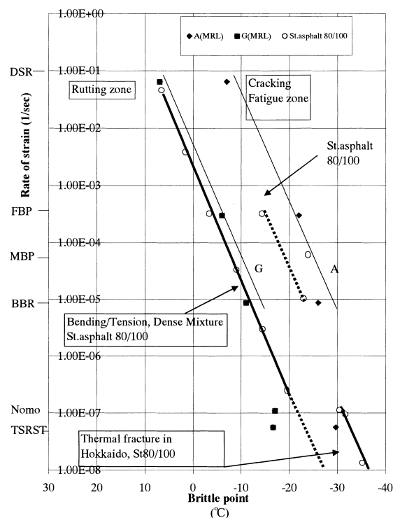
Fig. 10 Relationships between Brittle Point and Rate of Strain for Different Test Methods
