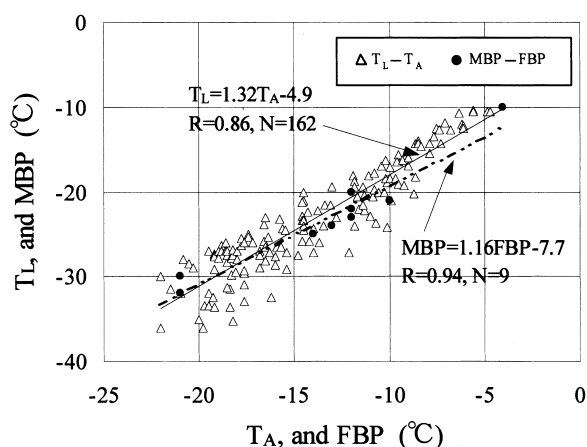
Fig. 9 Relationships between MBP, FBP, and Lowest Ambient Temperature ( T_L ) and Average Daily Temperature ( T_A )
