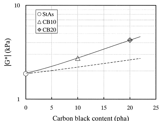
Fig. 8 Changes of |G^*| at 60°C Caused by Adding Carbon Black
