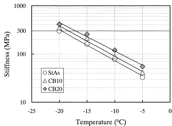
a) Stiffness
