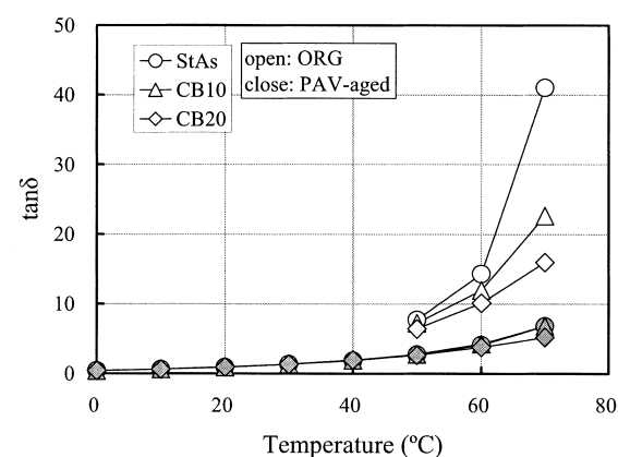
Fig. 3 \tan\delta of ORG and PAV-aged Samples with and without Carbon Black by DSR
