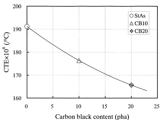
Fig. 7 CTE of TFO-aged Sample with and without Carbon Black
