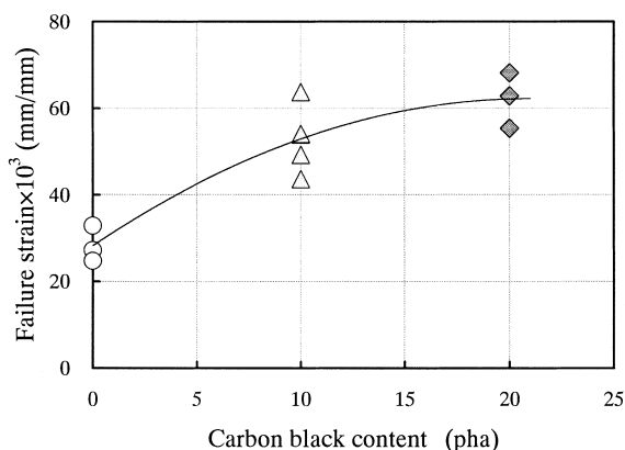
Fig. 6 Effects of Carbon Black on the Failure Strain of PAV-aged Samples by Destructive Bending Test
