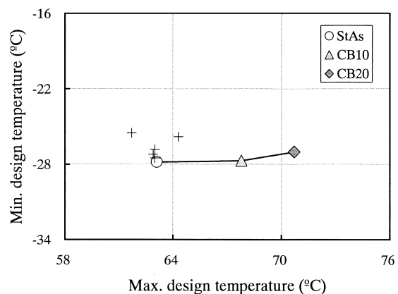
Fig. 5 Changes in PG Caused by Adding Carbon Black
