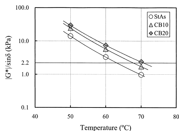
Fig. 2 |G^*|/\sin\delta of TFO-aged Samples with and without Carbon Black by DSR
