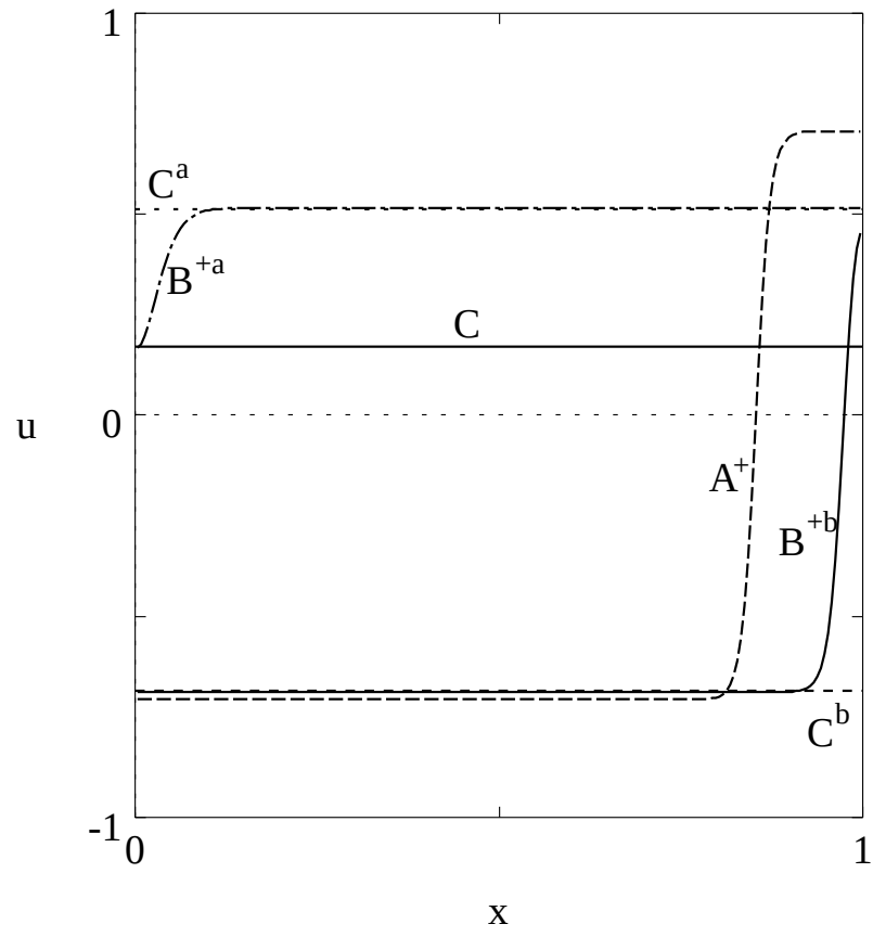
Figure 1: Wave profiles of stationary solutions for the parameter values k = 0.5 , \varepsilon = 0.01 , \lambda = 0.12 , \mu = 0.06 .
