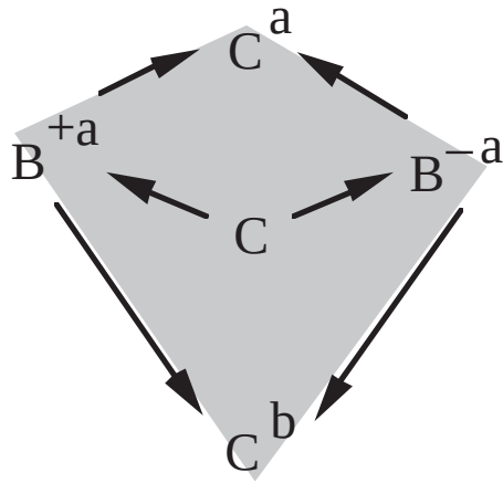
Figure 10: The flow to which \mathcal{A}_{\mathcal{M}}(\text{V}_+) is semi-conjugate.
