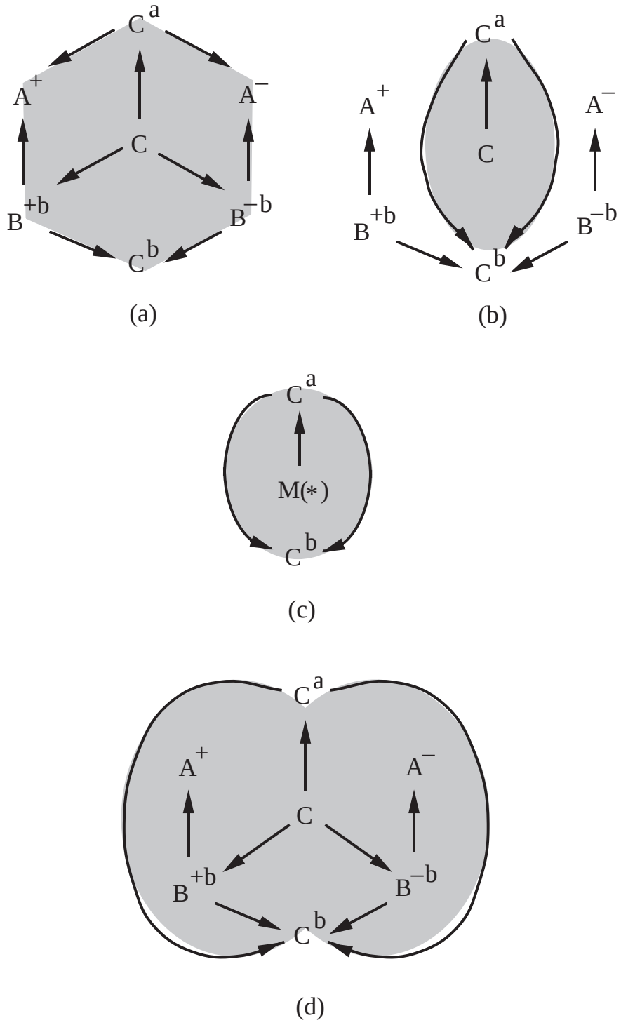
Figure 13: Three flows, to one of which \mathcal{A}_{\mathcal{M}}(\text{VII}_+) is semi-conjugate.
