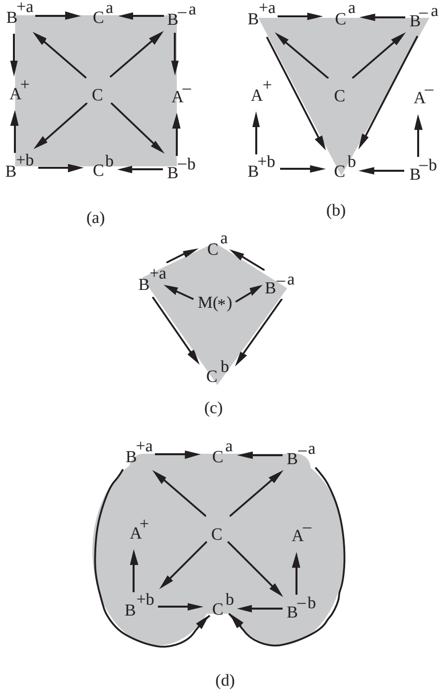
Figure 16: Three flows, to one of which \mathcal{A}_{\mathcal{M}}(\text{VIII}_+) is semi-conjugate.
