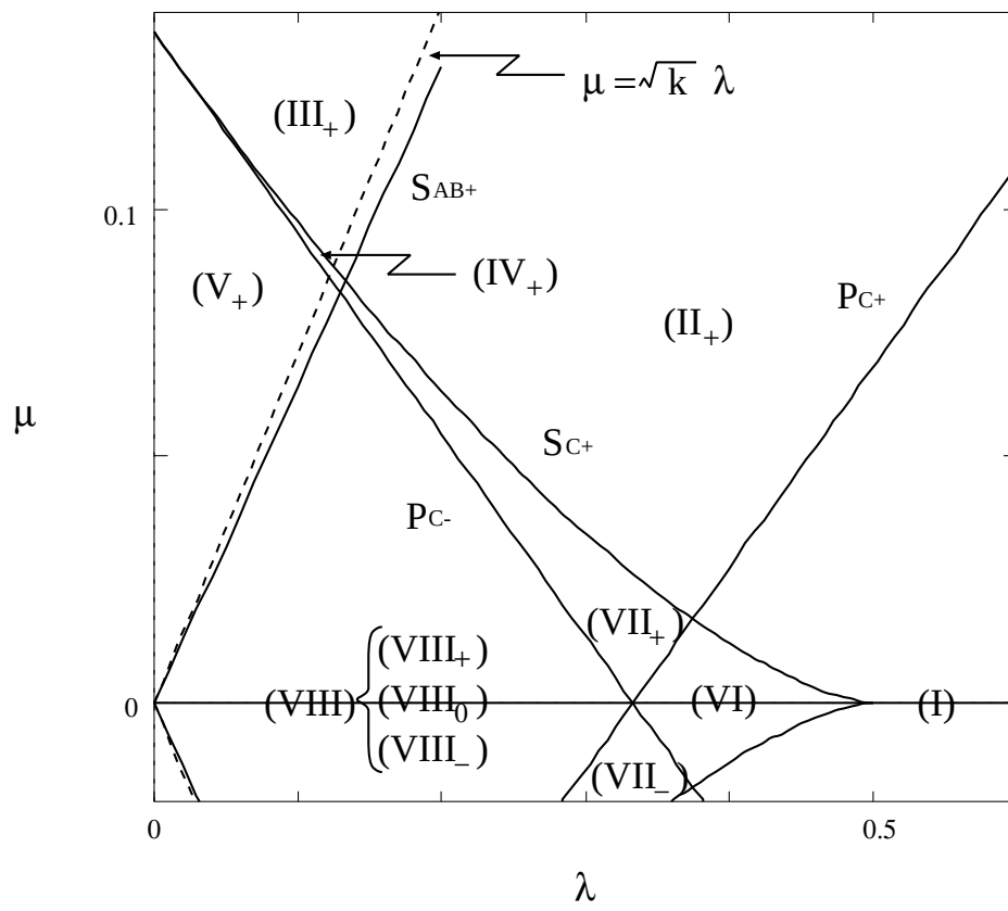
Figure 2: Bifurcation sets for the shadow system with k=0.5 .
