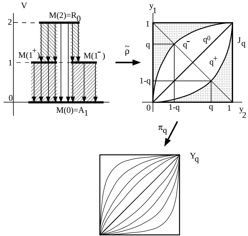
Figure 20: Map from the Morse decomposition onto J_q and Y_q .
