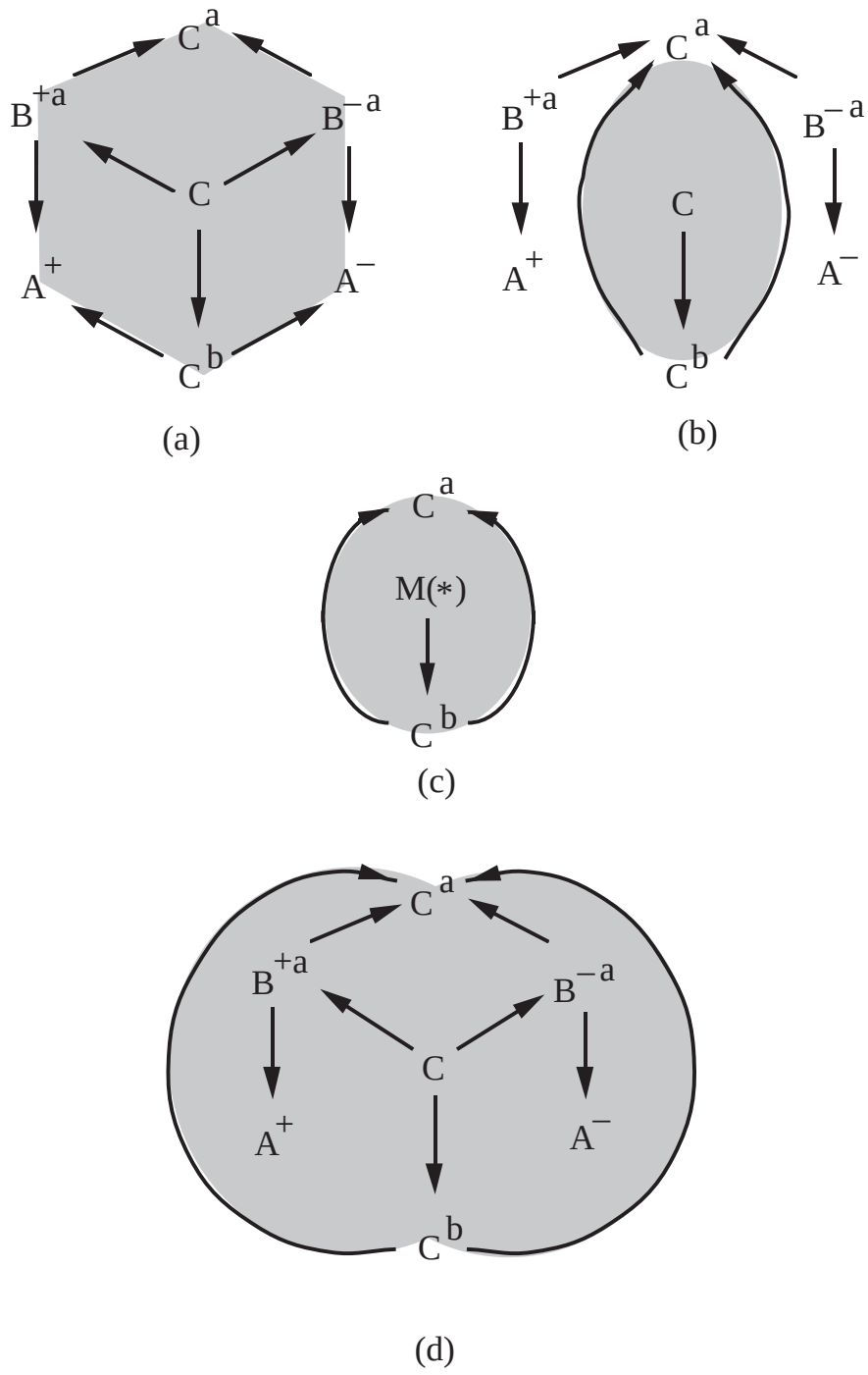
Figure 14: Three flows, to one of which \mathcal{A}_{\mathcal{M}}(\text{VII}_-) is semi-conjugate.
