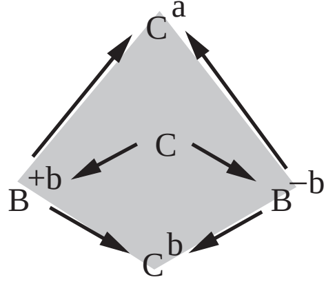
Figure 11: The flow to which \mathcal{A}_{\mathcal{M}}(V_-) is semi-conjugate.
