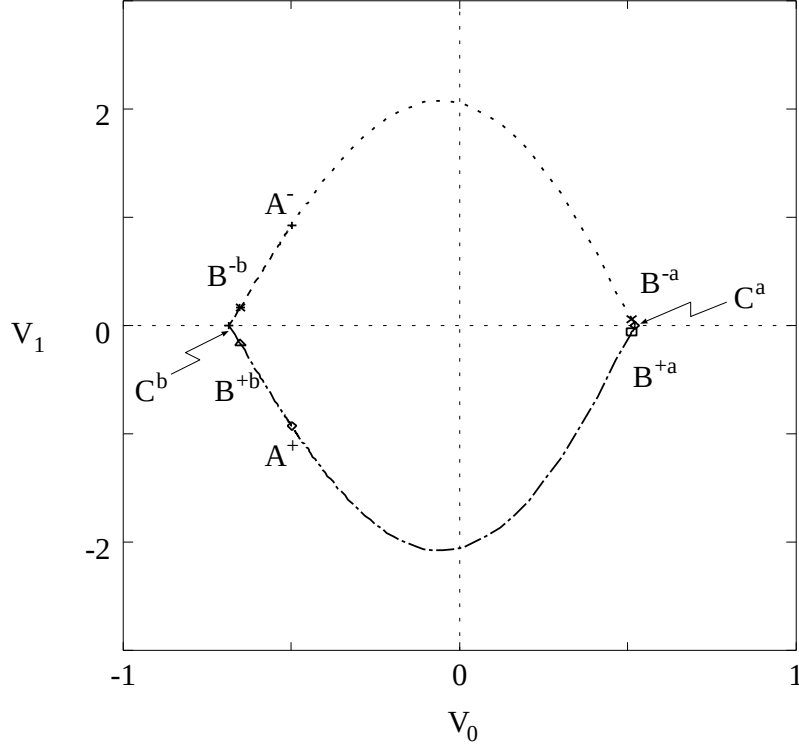
Figure 22: Projection of connections to (v_0, v_1) -space with k = 0.5 , \varepsilon = 0.01 , \lambda = 0.12 , \mu = 0.06
