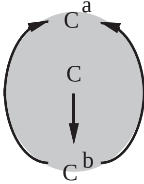
Figure 9: The flow to which \mathcal{A}_{\mathcal{M}}(\text{IV}_-) is semi-conjugate.
