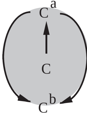
Figure 8: The flow to which \mathcal{A}_{\mathcal{M}}(\text{IV}_+) is semi-conjugate.
