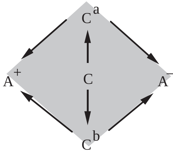
Figure 12: A flow to which \mathcal{A}_{\mathcal{M}}(VI) is semi-conjugate.
