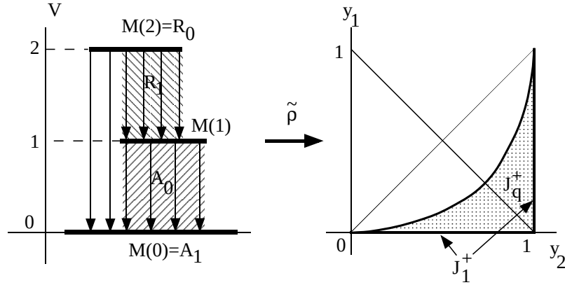
Figure 19: Map from the Morse decomposition onto \mathcal{D} .
