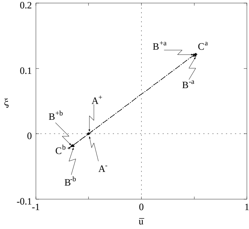
Figure 21: Projection of connections to (\bar{u}, \xi) -space with k = 0.5 , \varepsilon = 0.01 , \lambda = 0.12 , \mu = 0.06
