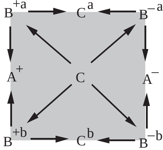
Figure 15: A flow to which \mathcal{A}_{\mathcal{M}}(\text{VIII}_0) is semi-conjugate.
