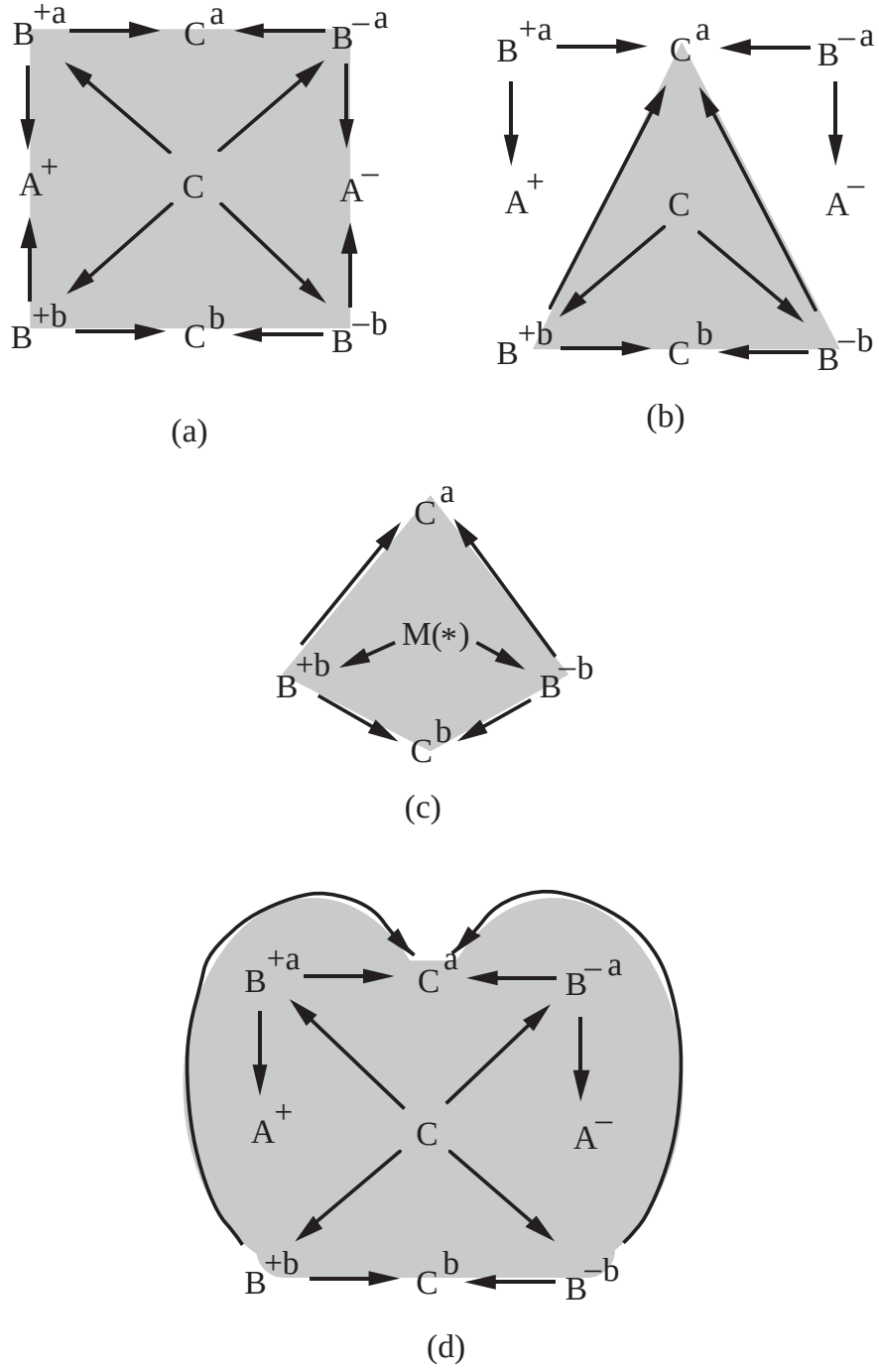
Figure 17: Three flows, to one of which \mathcal{A}_{\mathcal{M}}(\text{VIII}_-) is semi-conjugate.
