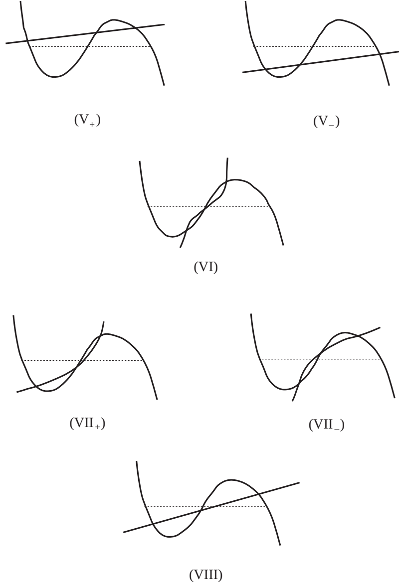
Figure 4: Qualitative aspects of the curves f(u, \xi) = 0 and g(u, \xi) = 0 in each of the parameter regions (continued).
