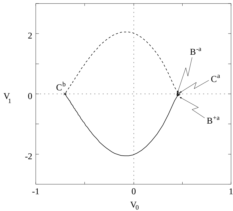
Figure 23: Projection of connections to (v_0, v_1) -space with k = 0.5 , \varepsilon = 0.01 , \lambda = 0.12 , \mu = 0.08
