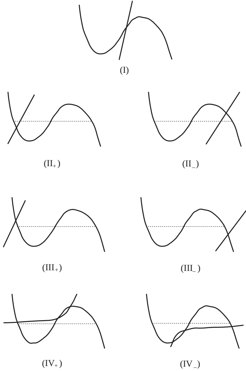
Figure 3: Qualitative aspects of the curves f(u, \xi) = 0 and g(u, \xi) = 0 in each of the parameter regions.
