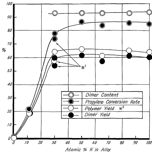
Fig. 1. Effect of the Composition of Alloy on the Propylene Dimerization.
