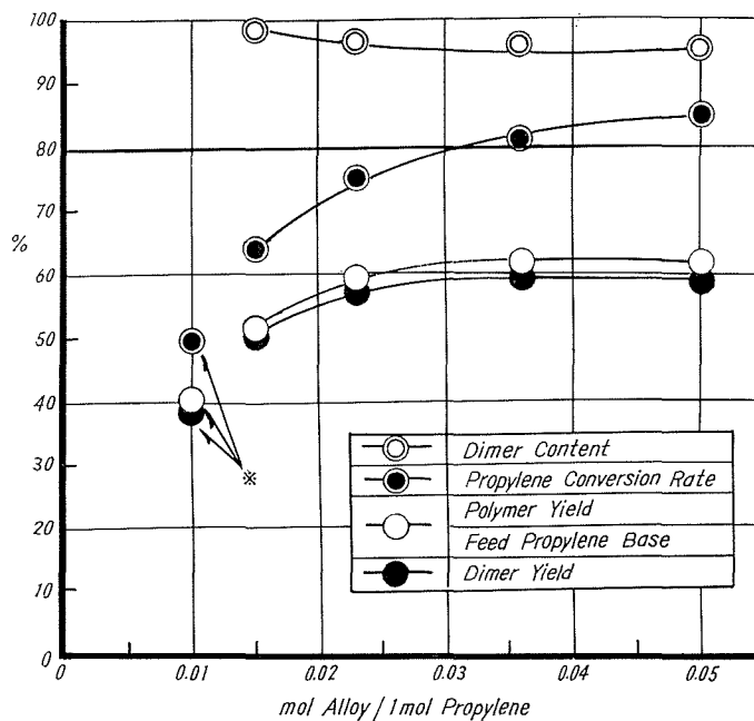
Fig. 3. Effect of the Alloy Catalyst Amount on the Propylene Dimerization.
