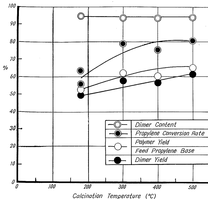
Fig. 4. Effect of Calcination Temperature of the Na-K 2 CO 3 Catalyst on the Propylene Dimerization. (Calc. Time: 3 hrs)
