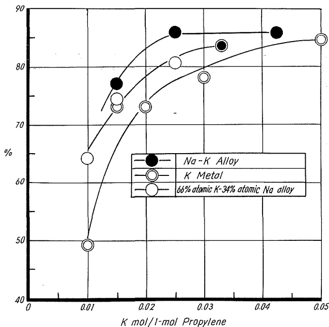
Fig. 2. Effect of the K-Base Catalyst Amount on the Propylene Conversion Rate.
