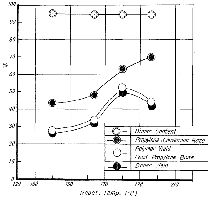
Fig. 5. Effect of Reaction Temperature on the Dimerization of Propylene.
