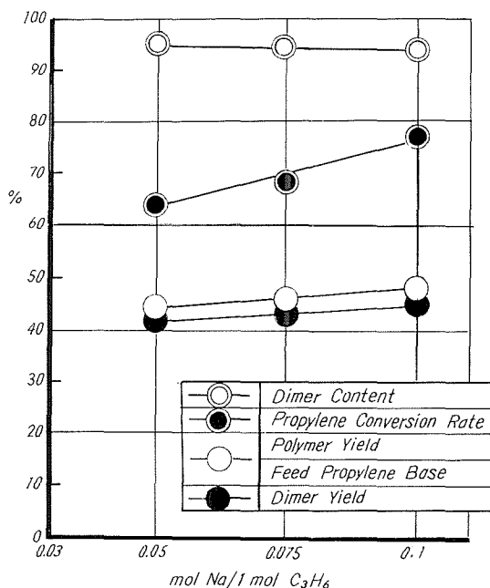
Fig. 7. Effect of Amount of Catalyst on the Dimerization of Propylene.
