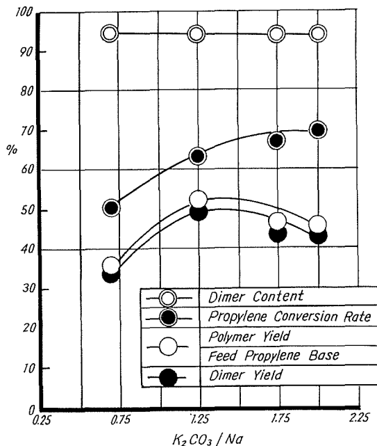
Fig. 6. Effect of Ratio \text{K}_2\text{CO}_3/\text{Na} in Catalyst on the Dimerization of Propylene.
