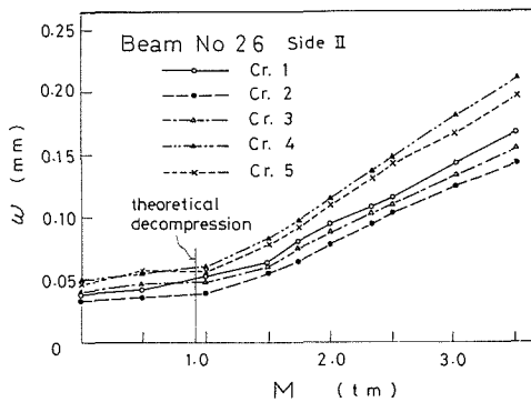
Fig. 7. Crack widths observed in static loading test after application of two hundreds thousand repetitions of loading.
