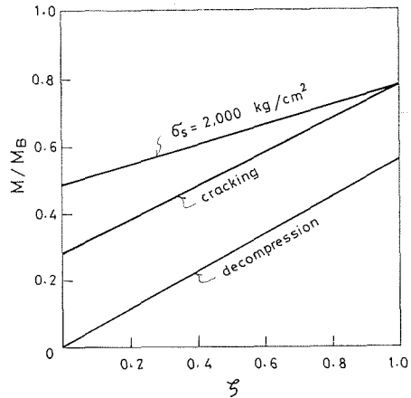
Fig. 12. Effect of prestressing on moments at decompression, cracking and steel stress of 2,000 kg/cm 2 in PRC beams.
