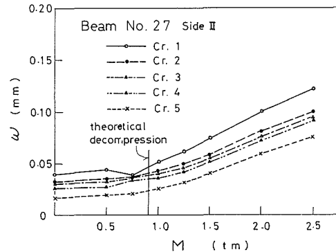
Fig. 8. Crack widths observed in static loading test after application of two hundreds thousand repetitions of loading.
