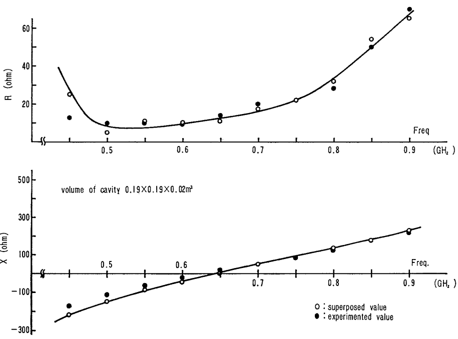
Fig. 12 First mode resonance for the uni pole
