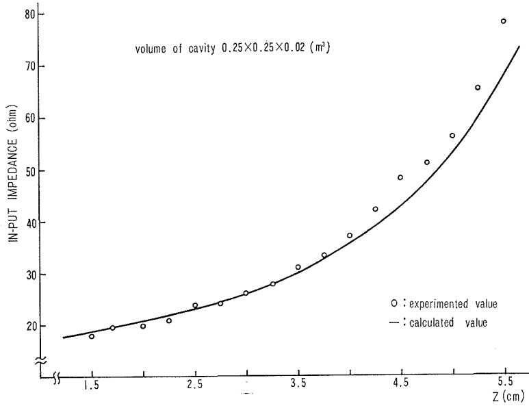
Fig. 7 In-put_impedence for (z)
