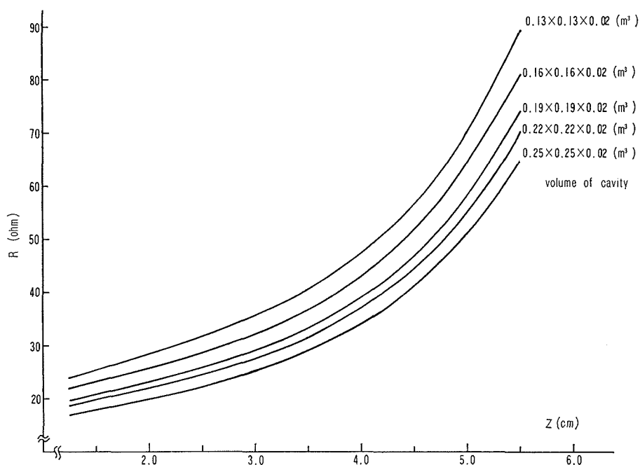
Fig. 6 In-put impedance for the position of off-set ( z )
