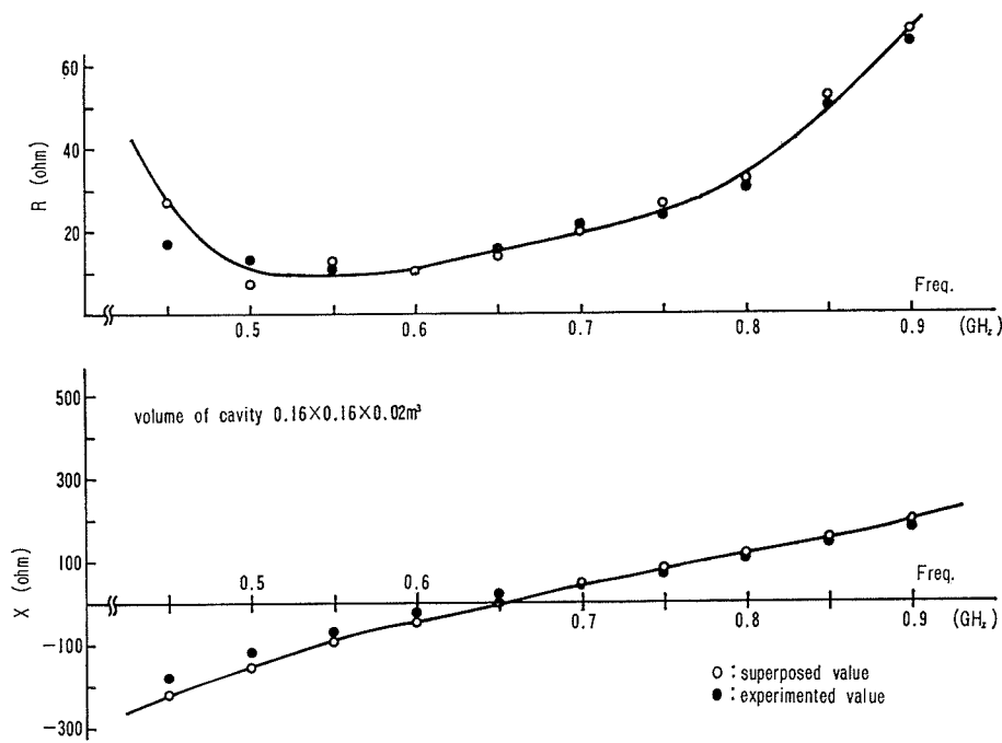
Fig. 11 First mode resonance for the uni pole
