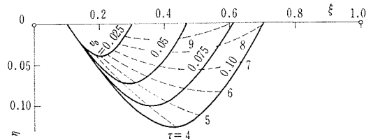
Fig. 4 The motion of a mass point colliding with a cable ( p_0=0.01 , \mu=0.3 ; \alpha_0=30^\circ )
