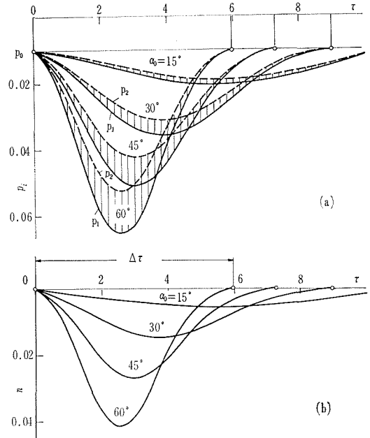
Fig. 3 The variation of the cable tension and reaction ( \mu=0.3 ; v_0=0.075 )
