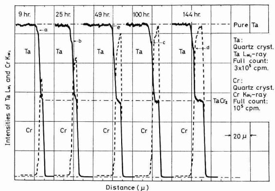
Fig. 4 EPMA patterns from chromized Ta sheet
