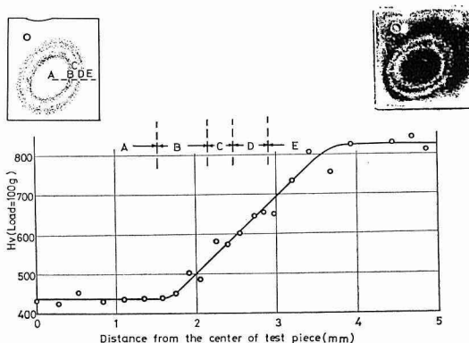
Fig. 6 Change in hardness in various depths of chromized Ta sheet
