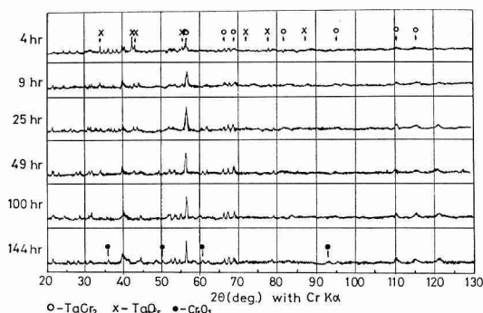
Fig. 7 X-ray diffraction patterns from the oxidized Ta for 15 min at 1000°C which was chromized with various times
