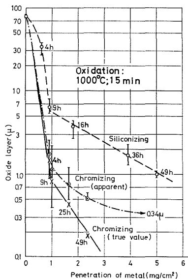
Fig. 12 Comparison of oxidation of chromized Ta with siliconized one
