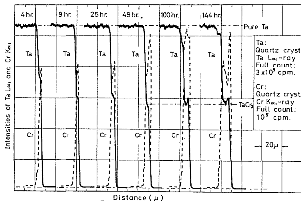
Fig. 8 EPMA patterns from oxidized Ta sheets which were chromized
