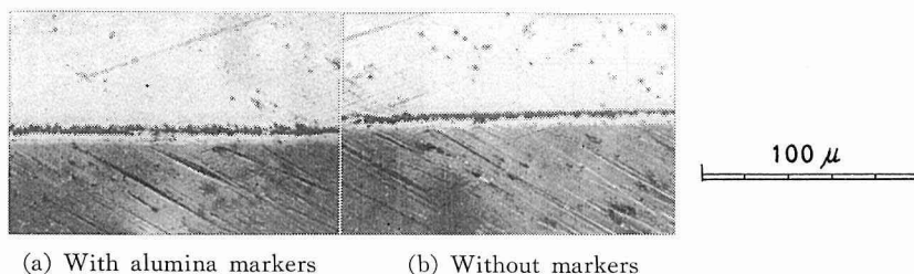
Photo 2 Markers experiment on chromizing of Ta sheet
