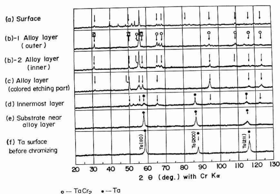
Fig. 5 X-ray diffraction patterns from the chromized Ta sheet in the various depths as well as pure Ta sheet
