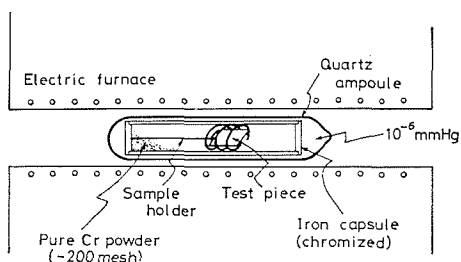
Fig. 1 Schematic presentation of chromizing ampoule and its furnace
