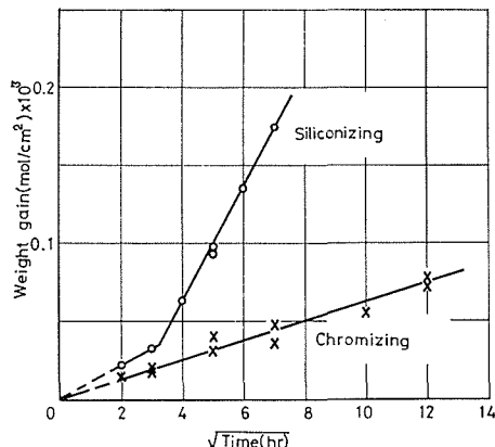
Fig. 11 Comparison of chromizing with siliconizing
