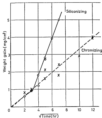
Fig. 10 Comparison of chromizing with siliconizing
