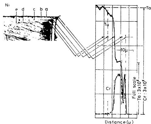
Fig. 9 Details of alloy layers containing oxide scale
