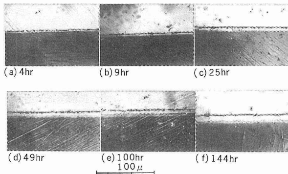
Photo 1 Sectional views of chromized Ta sheets at 1000°C; upper part: plated Ni, lower part: Ta, intermediate alloy layer: Ta-Cr alloy
