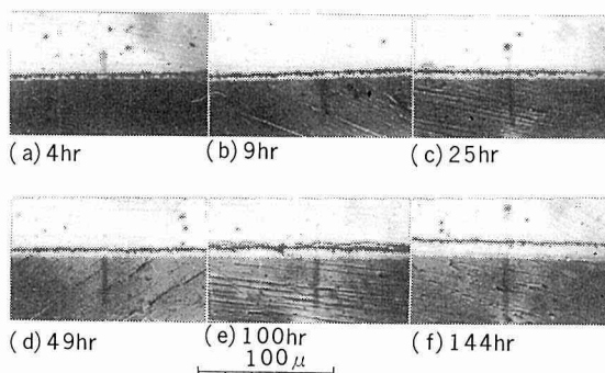
Photo. 3 Sectional views of oxidized Ta sheets after chromizing with various times ; upper part : plated Ni, lower part : Ta, intermediate black part : oxide, intermediate white layer : Ta-Cr alloy
