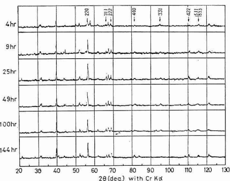
Fig. 3 X-ray diffraction ptners from the surface of chromized Ta sheets with various times at 1000°C
