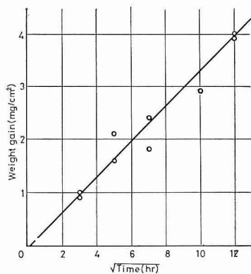
Fig. 2 Chromizing of Ta sheet at 1000°C
