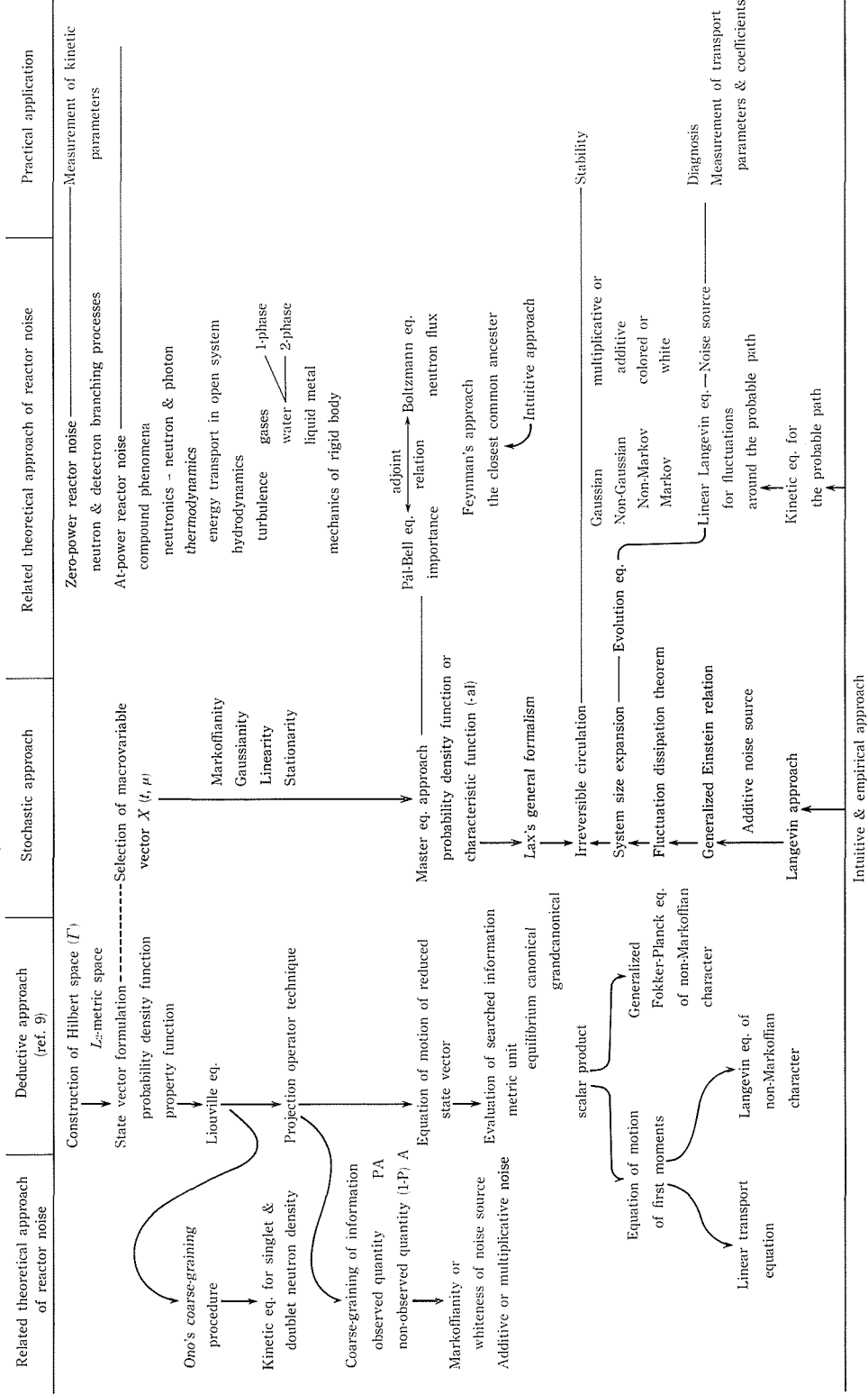
Fig. 1. Schematic Map Correlating the Basic Reactor Noise Theory to the Statistical Mechanics.
