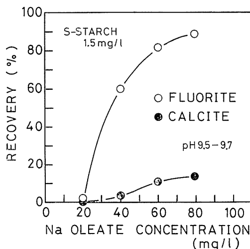
Fig. 12. Effect of sodium oleate concentration on flotation of fluorite-calcite mixture.
