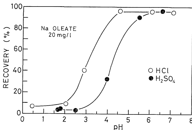
Fig. 3. Effect of HCl and H_2SO_4 on flotation of fluorite.
