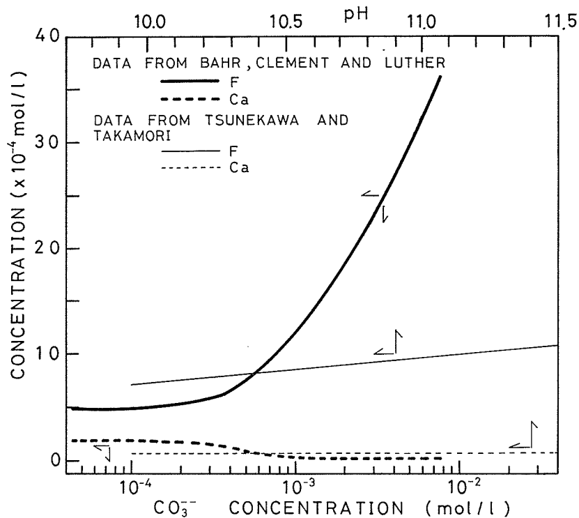
Fig. 5. Influence of \text{Na}_2\text{CO}_3 and \text{KOH} on fluorite in water.
