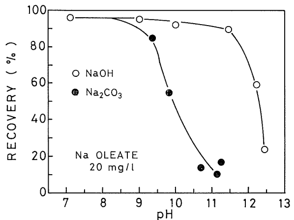
Fig. 4. Effect of NaOH and \text{Na}_2\text{CO}_3 on flotation of fluorite.
