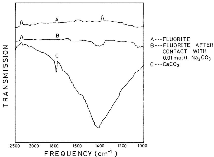
Fig. 6. Infrared spectra.
