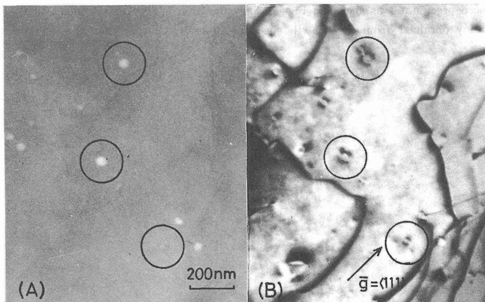
Fig. 7 Void contrast in Cu-Ni alloy irradiated to 7 dpa at 573 K. (A) absorbed condition, and (B) diffracted condition. Note the coherent strain field around void.
