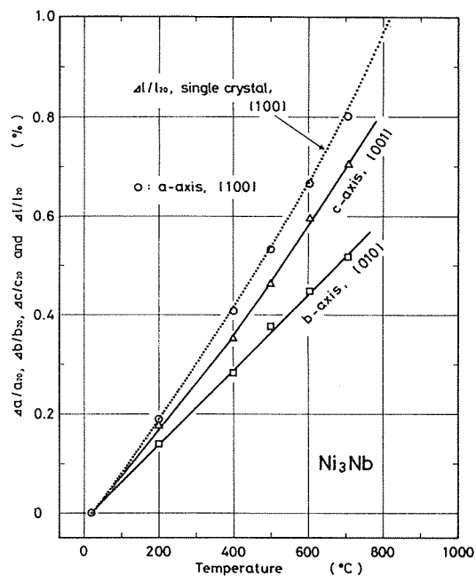
Fig. 3 Lattice thermal and dilatometric expansion of \delta phase.
