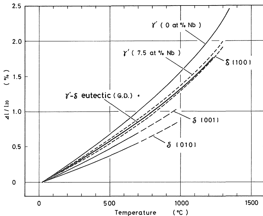
Fig. 4 Thermal expansion in the growth direction of directionally solidified \gamma' - \delta eutectic alloy and its constituent phases.
