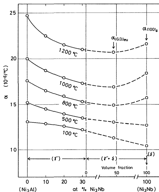
Fig. 5 Relation between coefficient of thermal expansion and composition of pseudo-binary alloys.
