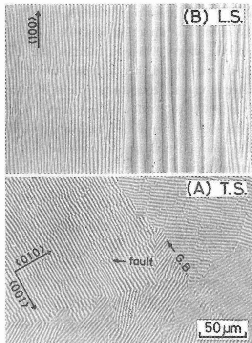
Photo. 1 Microstructures of directionally solidified \gamma' - \delta eutectic alloy.
