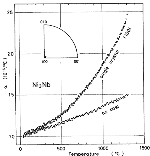
Fig. 2 Temperature dependence of thermal expansion coefficient of \delta phase.
