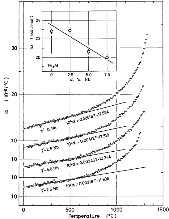
Fig. 1 Temperature dependence of thermal expansion coefficient ( \alpha ) and composition dependence of vacancy formation energy ( E_f ) for \gamma' phases.
