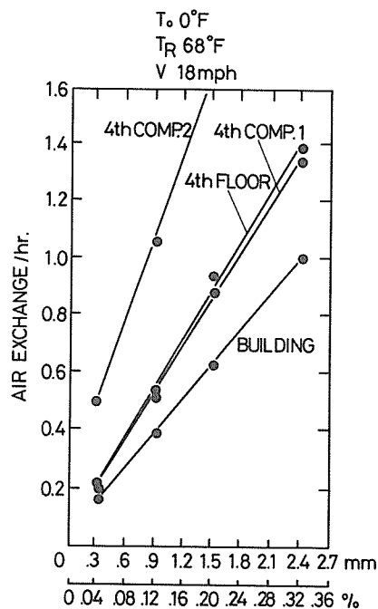
Figure 3. Relationship between the air change per hour data and building envelope porosity under 18 mph wind condition
