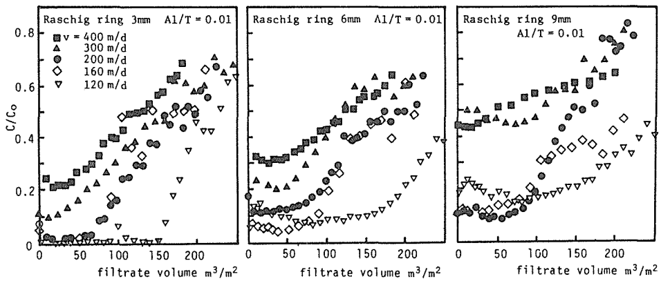
Fig.6 Fig.7 Fig.8 Variation of Raschig ring outflow concentration with filtration time
