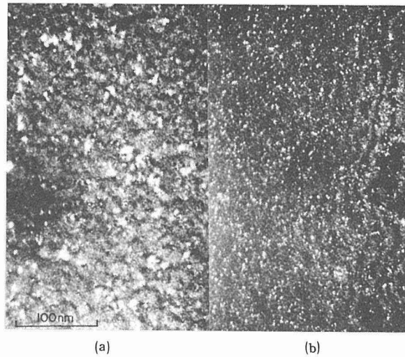
Fig. 14 Difference in clustered defect formation between (a) bulk and (b) thin foil irradiation of nickel at room temperature. Both 6 \times 10^{17} \text{ n/cm}^2 .
