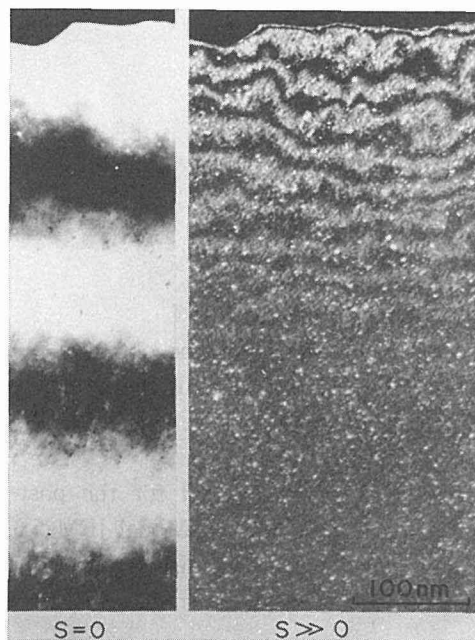
Fig. 5 Measurement of the number density of defects. The case of Ni, 7.7 \times 10^{17} \text{ n/cm}^2 . Specimen thickness is measured from the equal thickness fringes on the left, and areal number density is obtained from the weak beam electron microscope image on the right.
