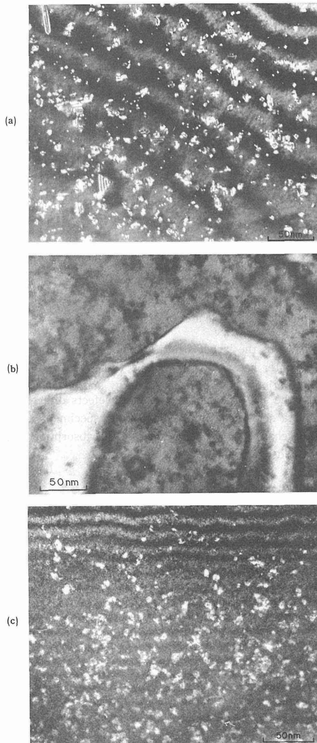
Fig. 9 Defect structures suggesting the existence of sub-cascade damage by D-T neutrons. (a) gold, 3.6 \times 10^{17} \text{ n/cm}^2 , (b) \text{Cu}_3\text{Au} , 1.8 \times 10^{17} \text{ n/cm}^2 , and (c) Ge, 7.9 \times 10^{17} \text{ n/cm}^2 , all irradiated at room temperature.
