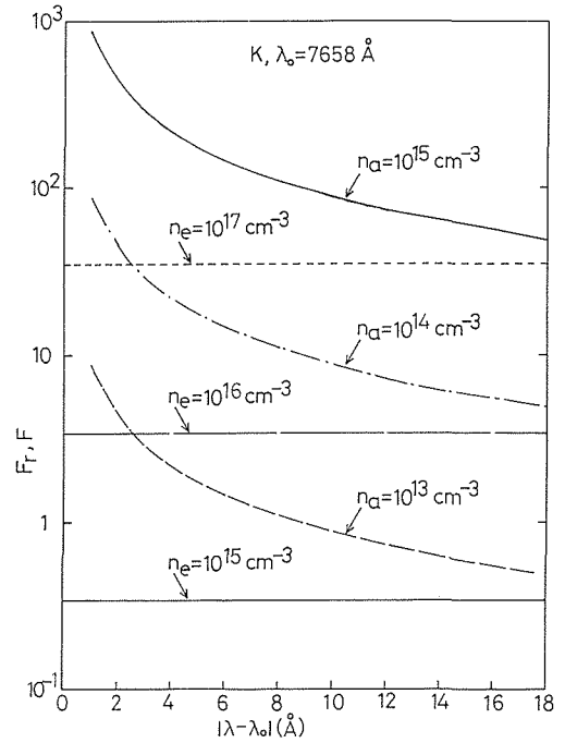
Fig.2 F_r and F_c as a function of |\lambda - \lambda_0| for \Delta\lambda \ll \lambda - \lambda_0 , l = 10^2 \text{ cm} , \lambda_0 = 7658 \text{ Å} ( K ).
