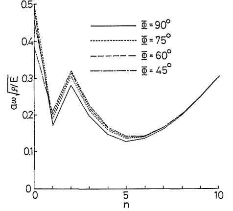
Fig. 3 Effect of half opening angles on fundamental frequencies ( h_c = h_s , L_c/a = 2 , h_c/a = 0.01 , \nu = 0.3 ).
