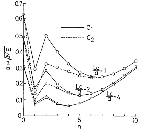
Fig. 5 Effect of thickness to radius ratios ( h_c/a ) on fundamental frequencies ( h_c = h_s , \Phi = 90^\circ , L_c/a = 2 , \nu = 0.3 ).
