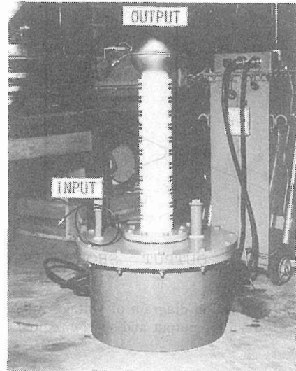
Photo. 2. Transformer encased in the tank filled with insulating oil.
