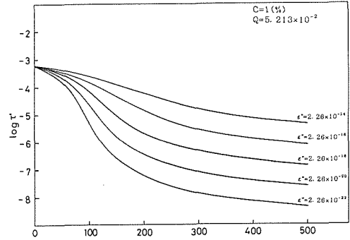
Fig. 5 Temperature dependency of normalized effective stress for various values of strain rate.
