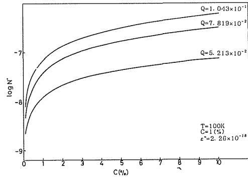
Fig. 7 Concentration dependency of normalized mobile dislocation density at 100 K.
