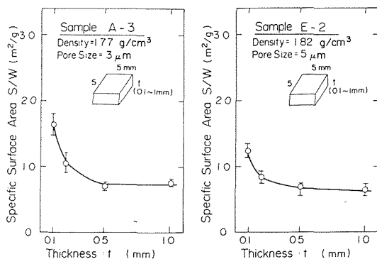
Fig. 4 The effects of the sample thickness on the specific surface areas
